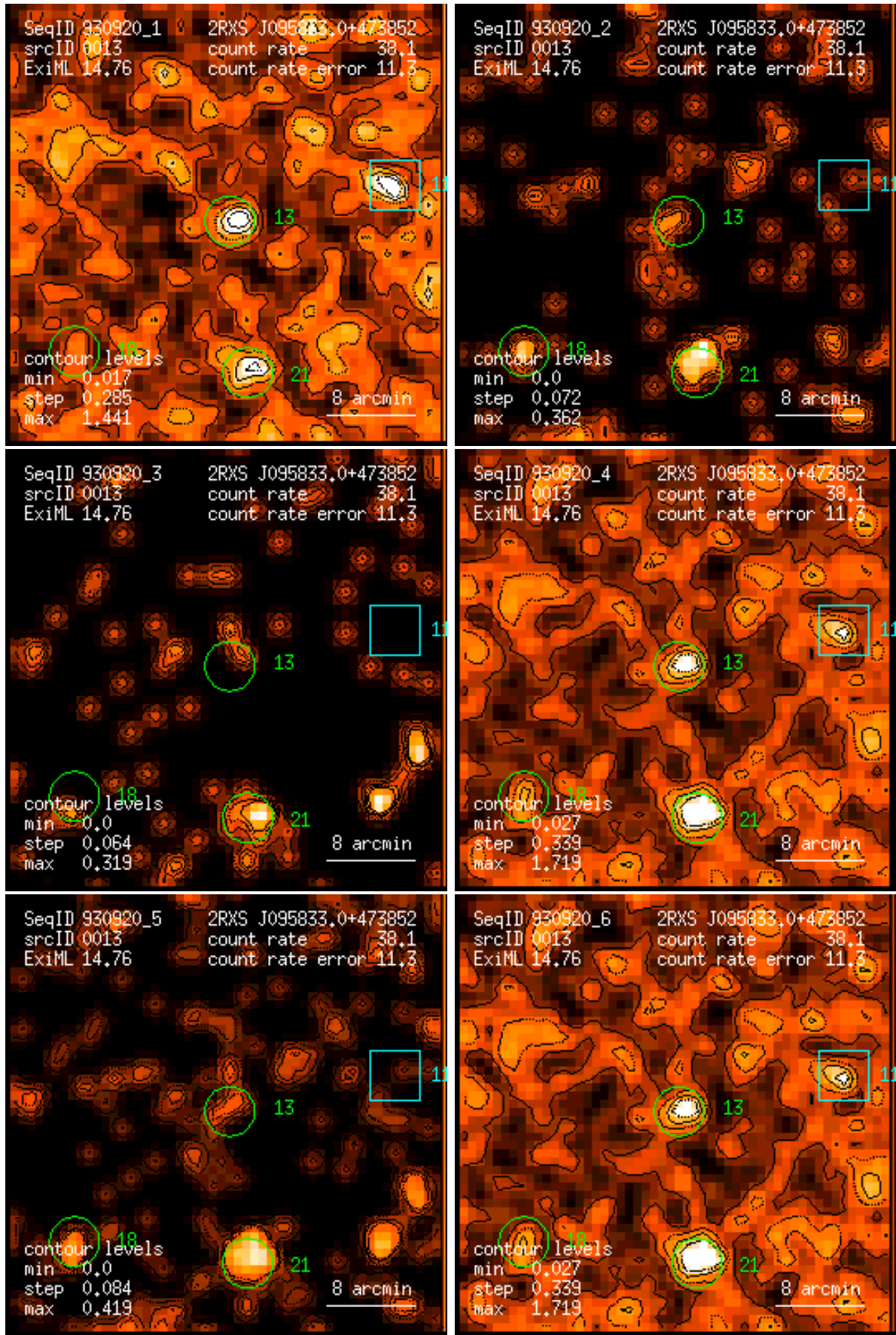
Figure 13: RASS 930920: detection 0013: band rate images, Gaussian filter: (1) PSPC channels 11 – 41, (2) 52 – 90, (3) 91 – 201, (4) 11 – 235, (5) 52 – 201, (6) 11 – 201. Broad band rates in counts/ks. Band rate contour levels in counts/ks/arcmin 2 .
