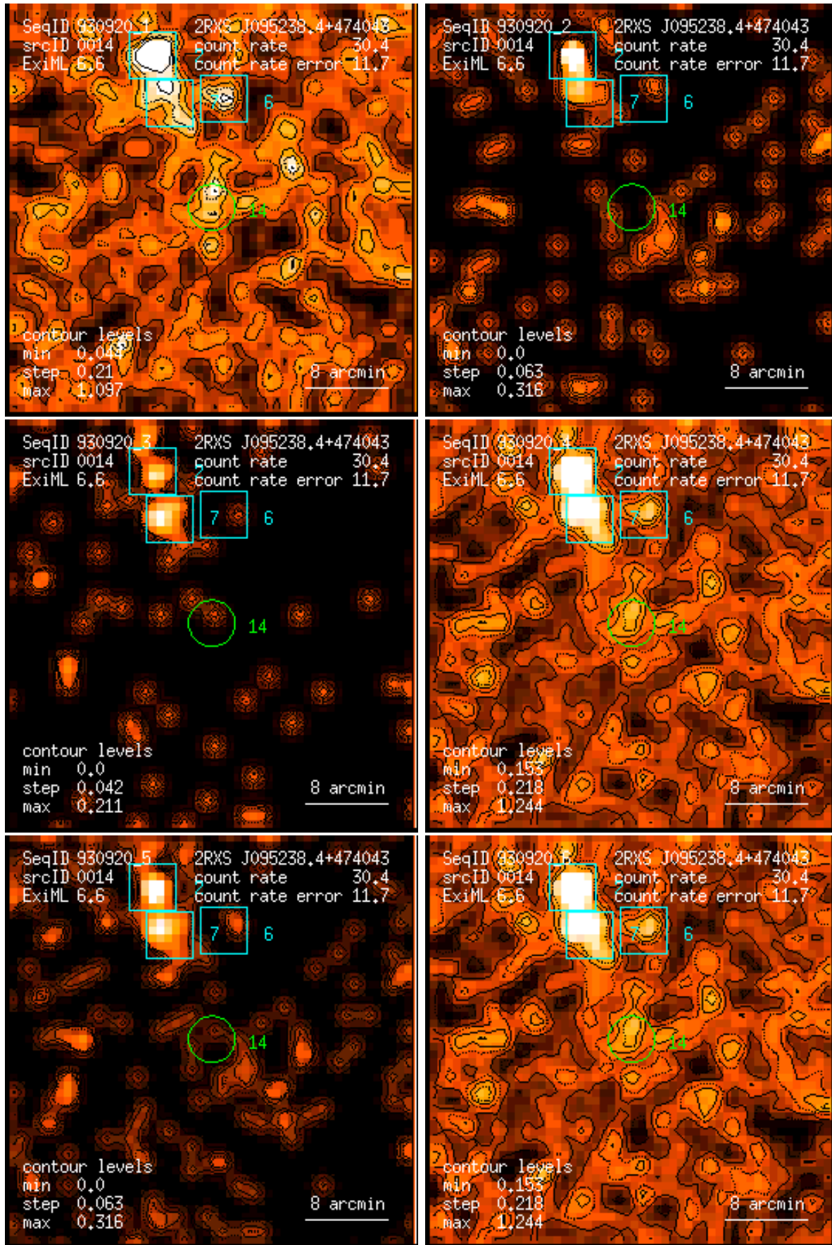
Figure 14: RASS 930920: detection 0014: band rate images, Gaussian filter: (1) PSPC channels 11 – 41, (2) 52 – 90, (3) 91 – 201, (4) 11 – 235, (5) 52 – 201, (6) 11 – 201. Broad band rates in counts/ks. Band rate contour levels in counts/ks/arcmin 2 .
