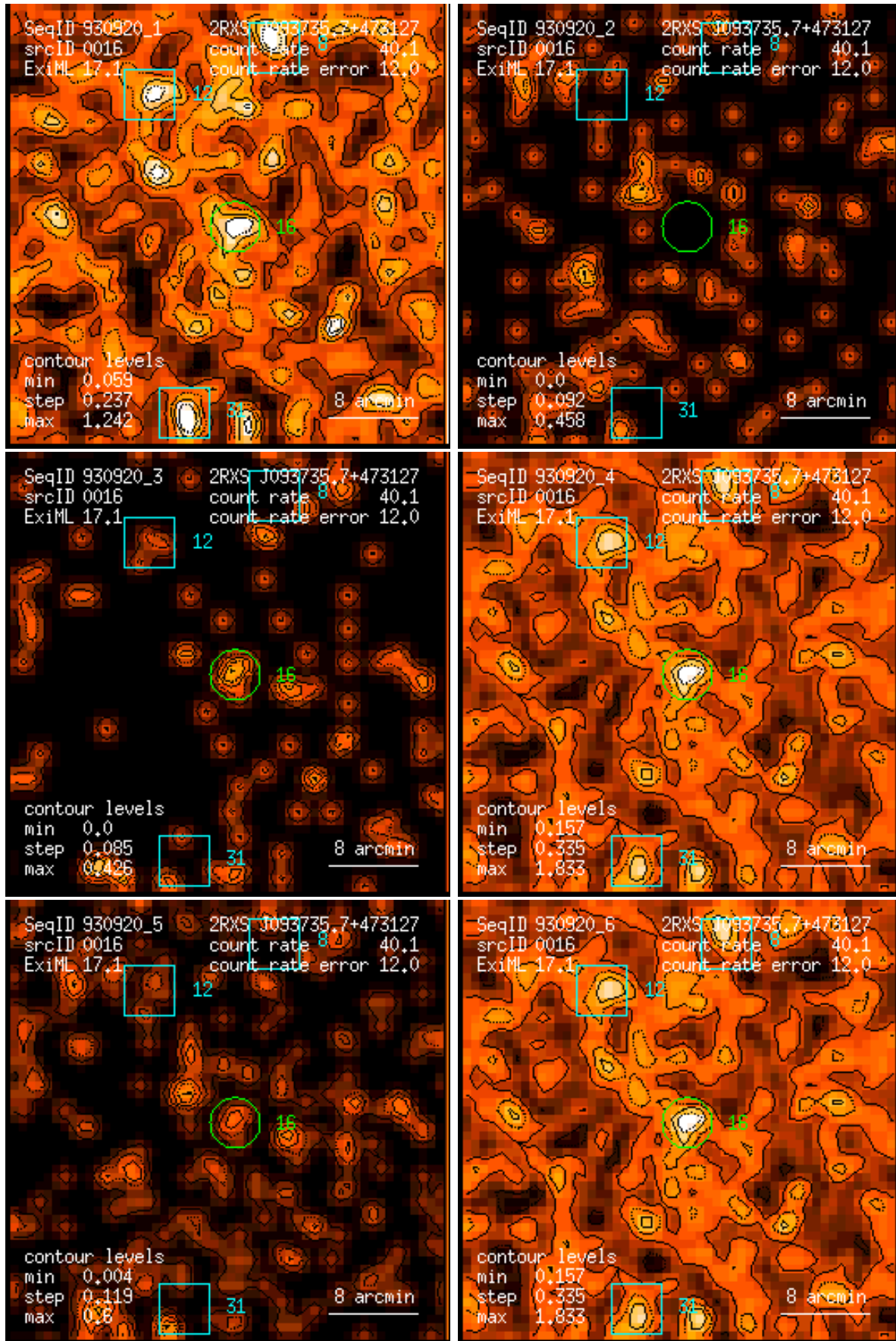
Figure 16: RASS 930920: detection 0016: band rate images, Gaussian filter: (1) PSPC channels 11 – 41, (2) 52 – 90, (3) 91 – 201, (4) 11 – 235, (5) 52 – 201, (6) 11 – 201. Broad band rates in counts/ks. Band rate contour levels in counts/ks/arcmin 2 .
