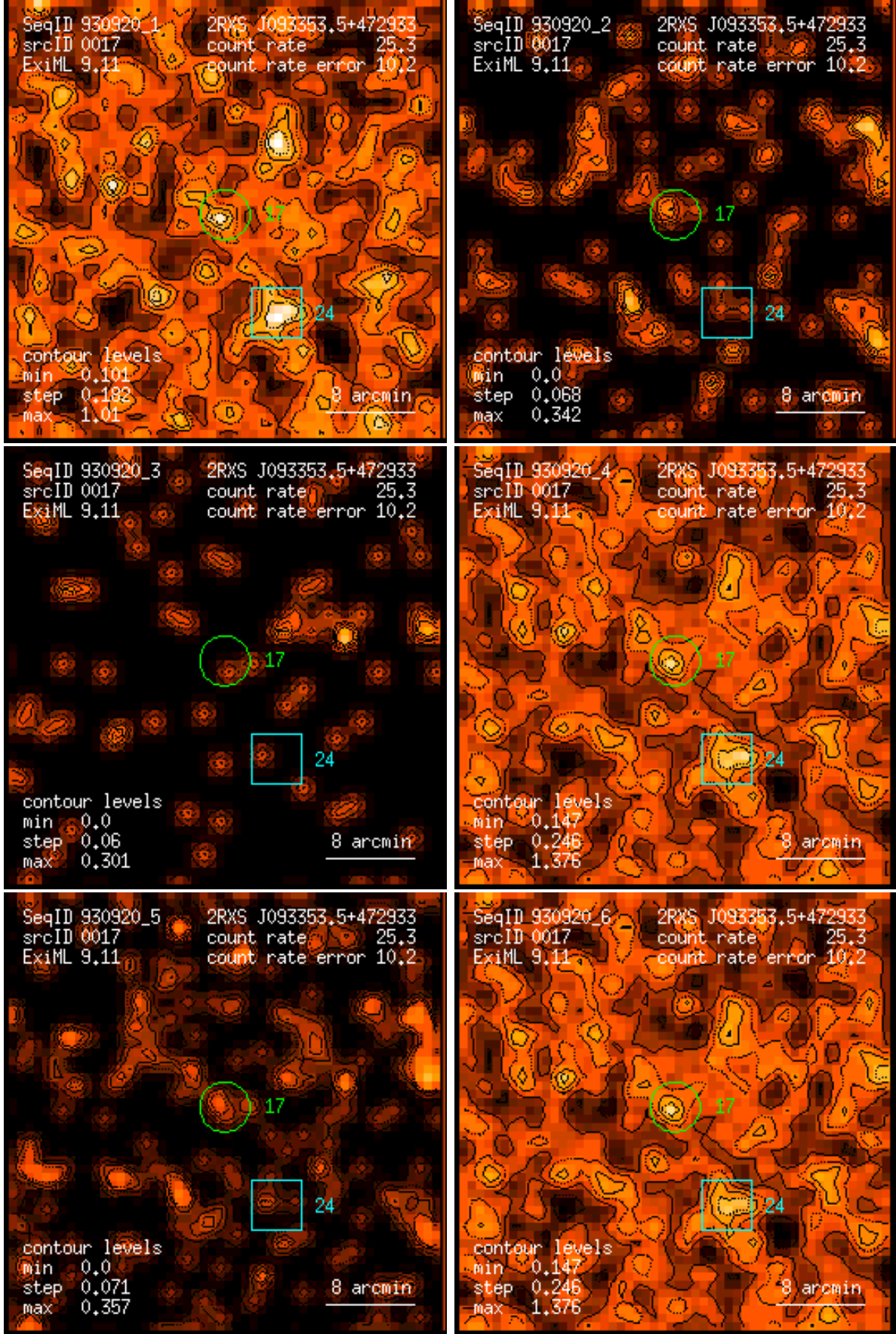
Figure 17: RASS 930920: detection 0017: band rate images, Gaussian filter: (1) PSPC channels 11 – 41, (2) 52 – 90, (3) 91 – 201, (4) 11 – 235, (5) 52 – 201, (6) 11 – 201. Broad band rates in counts/ks. Band rate contour levels in counts/ks/arcmin 2 .
