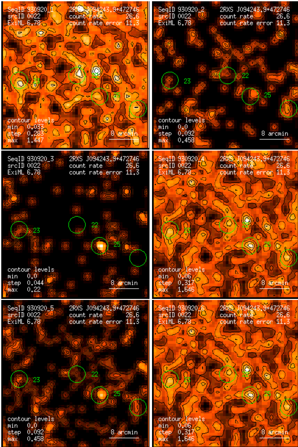
Figure 22: RASS 930920: detection 0022: band rate images, Gaussian filter: (1) PSPC channels 11 – 41, (2) 52 – 90, (3) 91 – 201, (4) 11 – 235, (5) 52 – 201, (6) 11 – 201. Broad band rates in counts/ks. Band rate contour levels in counts/ks/arcmin 2 .
