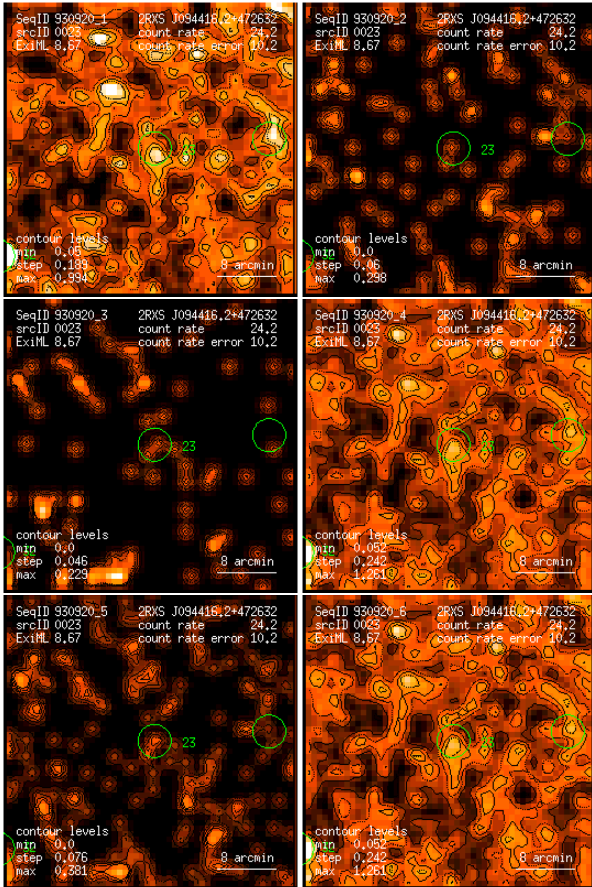
Figure 23: RASS 930920: detection 0023: band rate images, Gaussian filter: (1) PSPC channels 11 – 41, (2) 52 – 90, (3) 91 – 201, (4) 11 – 235, (5) 52 – 201, (6) 11 – 201. Broad band rates in counts/ks. Band rate contour levels in counts/ks/arcmin 2 .
