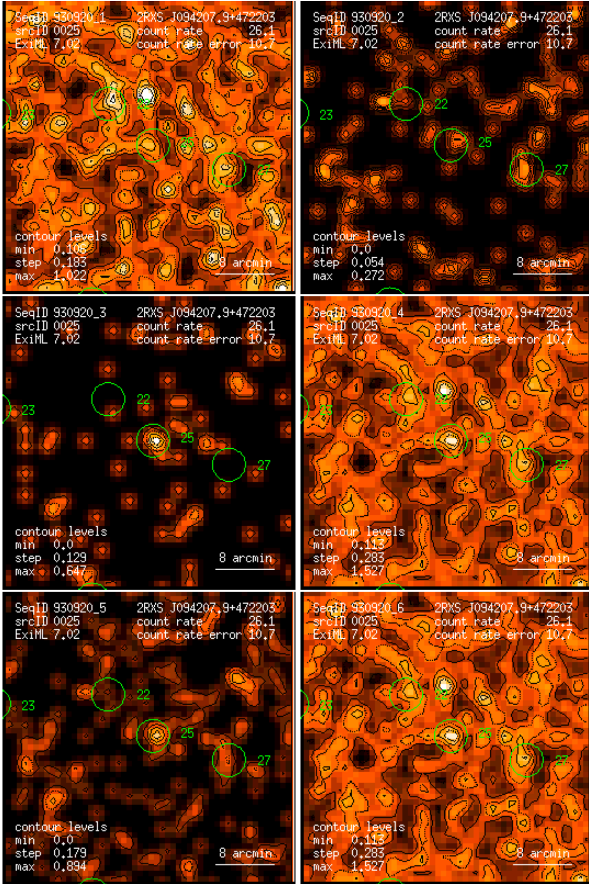
Figure 25: RASS 930920: detection 0025: band rate images, Gaussian filter: (1) PSPC channels 11 – 41, (2) 52 – 90, (3) 91 – 201, (4) 11 – 235, (5) 52 – 201, (6) 11 – 201. Broad band rates in counts/ks. Band rate contour levels in counts/ks/arcmin 2 .
