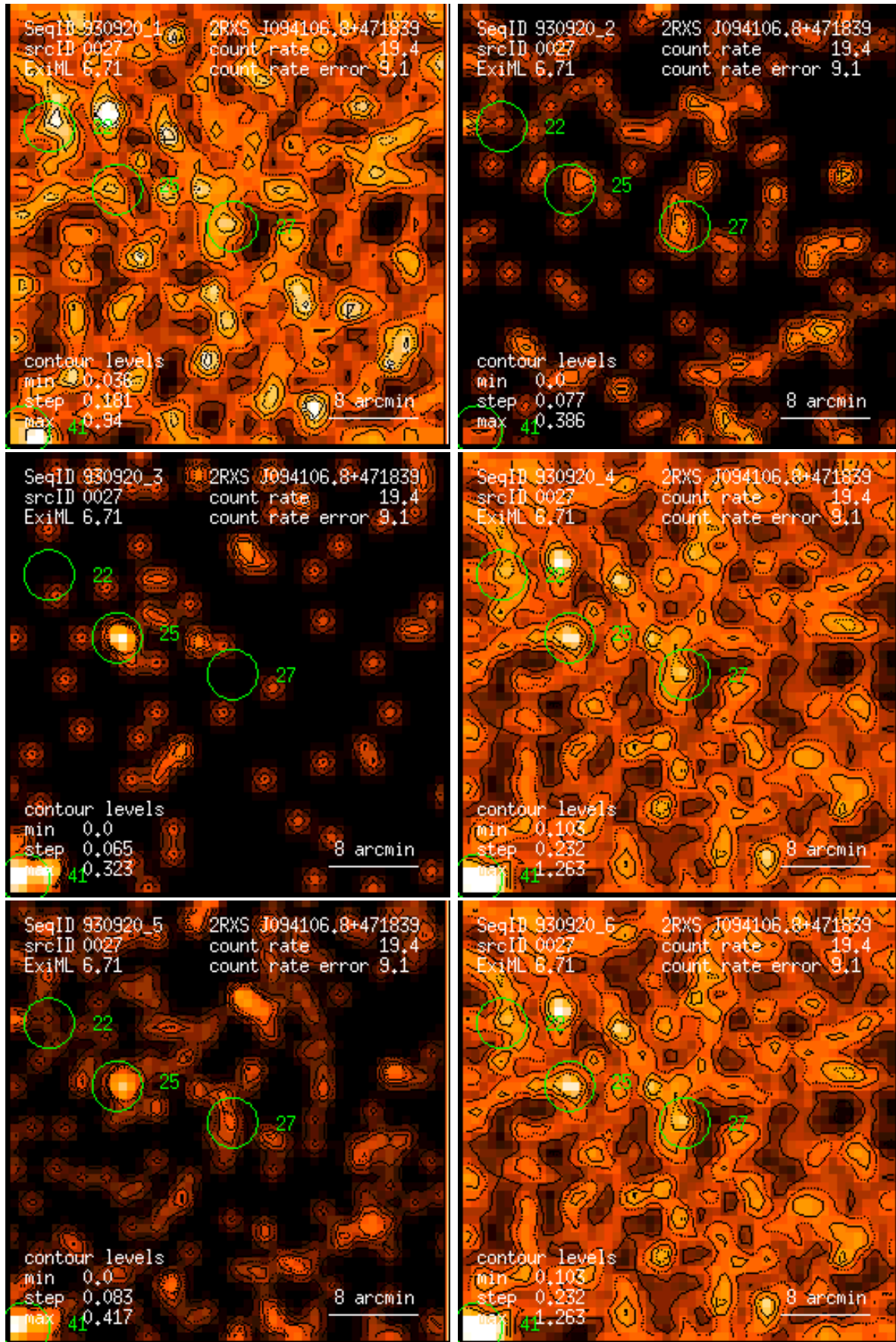
Figure 27: RASS 930920: detection 0027: band rate images, Gaussian filter: (1) PSPC channels 11 – 41, (2) 52 – 90, (3) 91 – 201, (4) 11 – 235, (5) 52 – 201, (6) 11 – 201. Broad band rates in counts/ks. Band rate contour levels in counts/ks/arcmin 2 .
