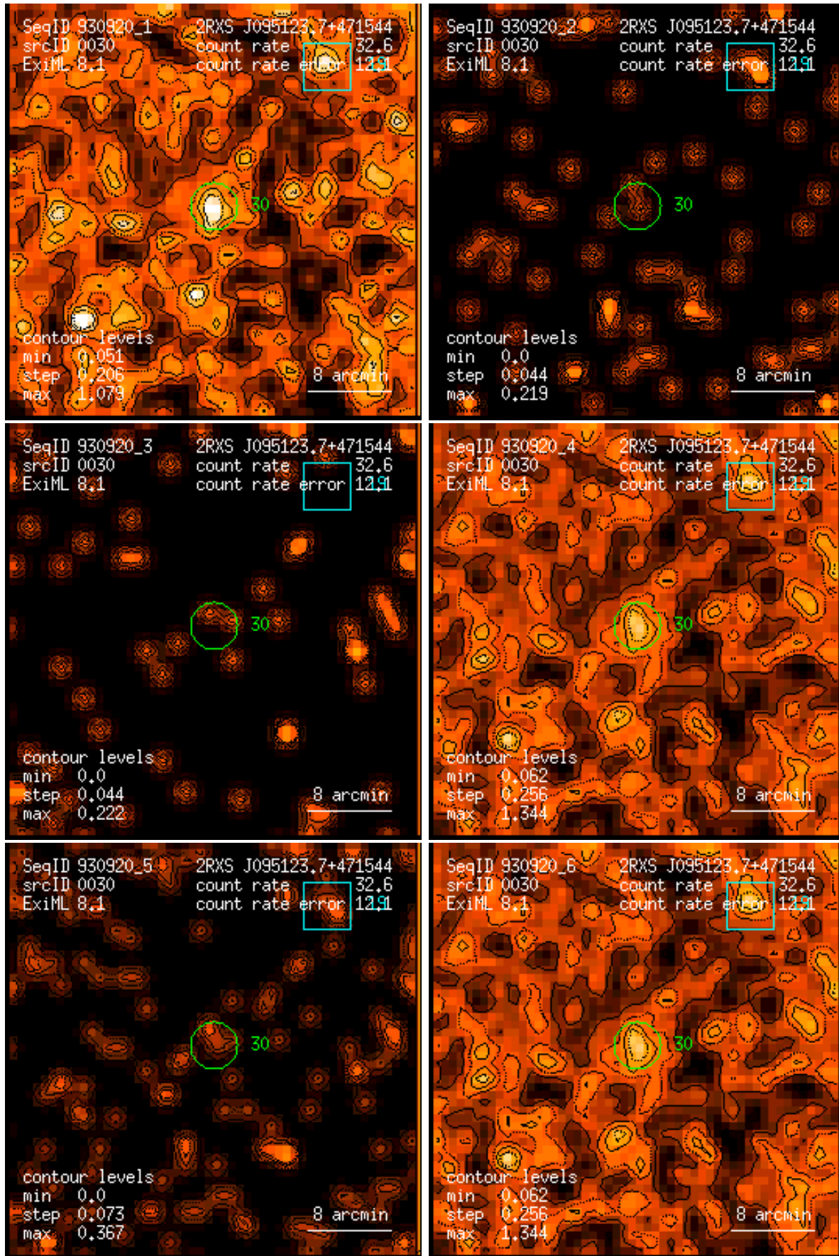
Figure 30: RASS 930920: detection 0030: band rate images, Gaussian filter: (1) PSPC channels 11 – 41, (2) 52 – 90, (3) 91 – 201, (4) 11 – 235, (5) 52 – 201, (6) 11 – 201. Broad band rates in counts/ks. Band rate contour levels in counts/ks/arcmin 2 .
