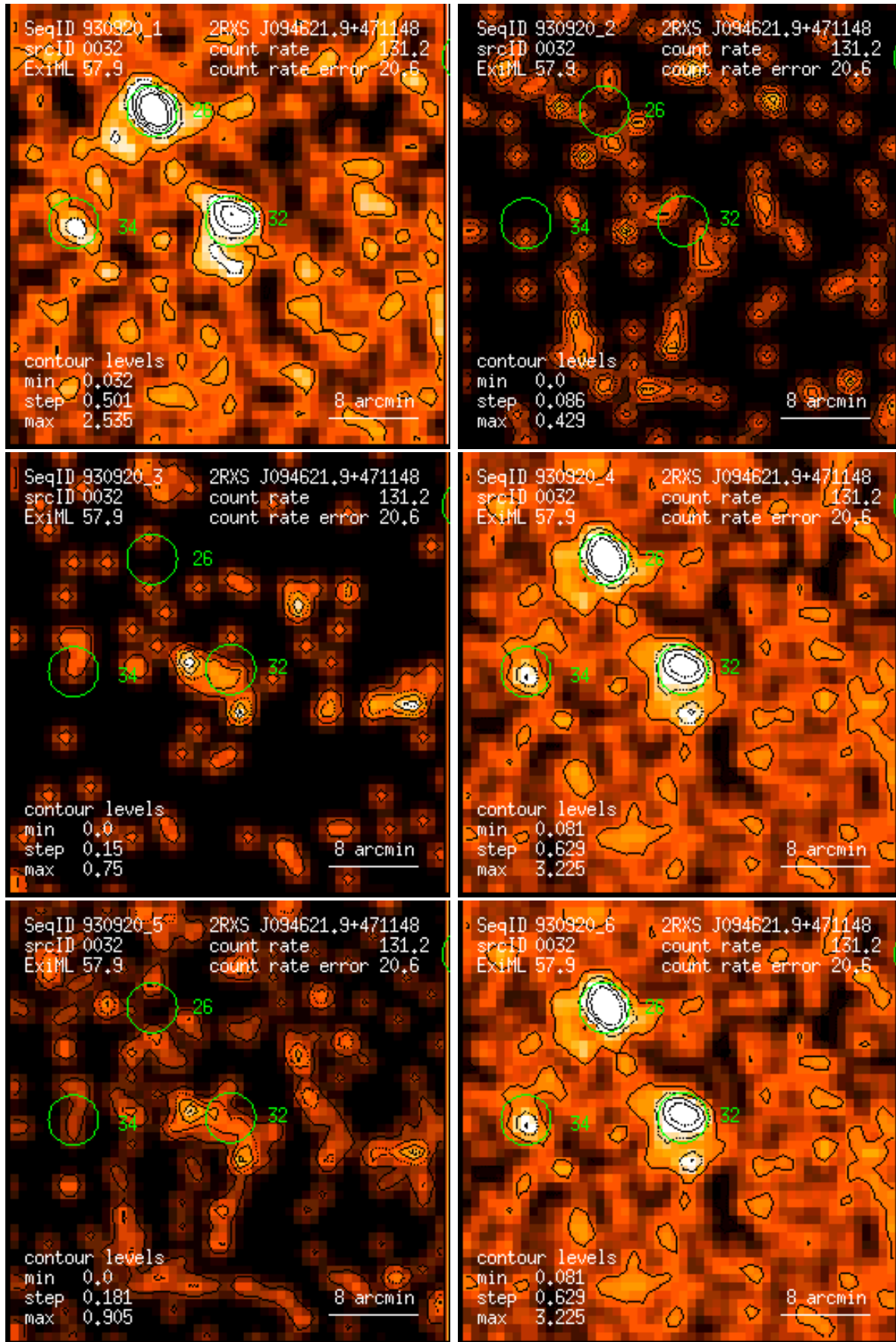
Figure 32: RASS 930920: detection 0032: band rate images, Gaussian filter: (1) PSPC channels 11 – 41, (2) 52 – 90, (3) 91 – 201, (4) 11 – 235, (5) 52 – 201, (6) 11 – 201. Broad band rates in counts/ks. Band rate contour levels in counts/ks/arcmin 2 .
