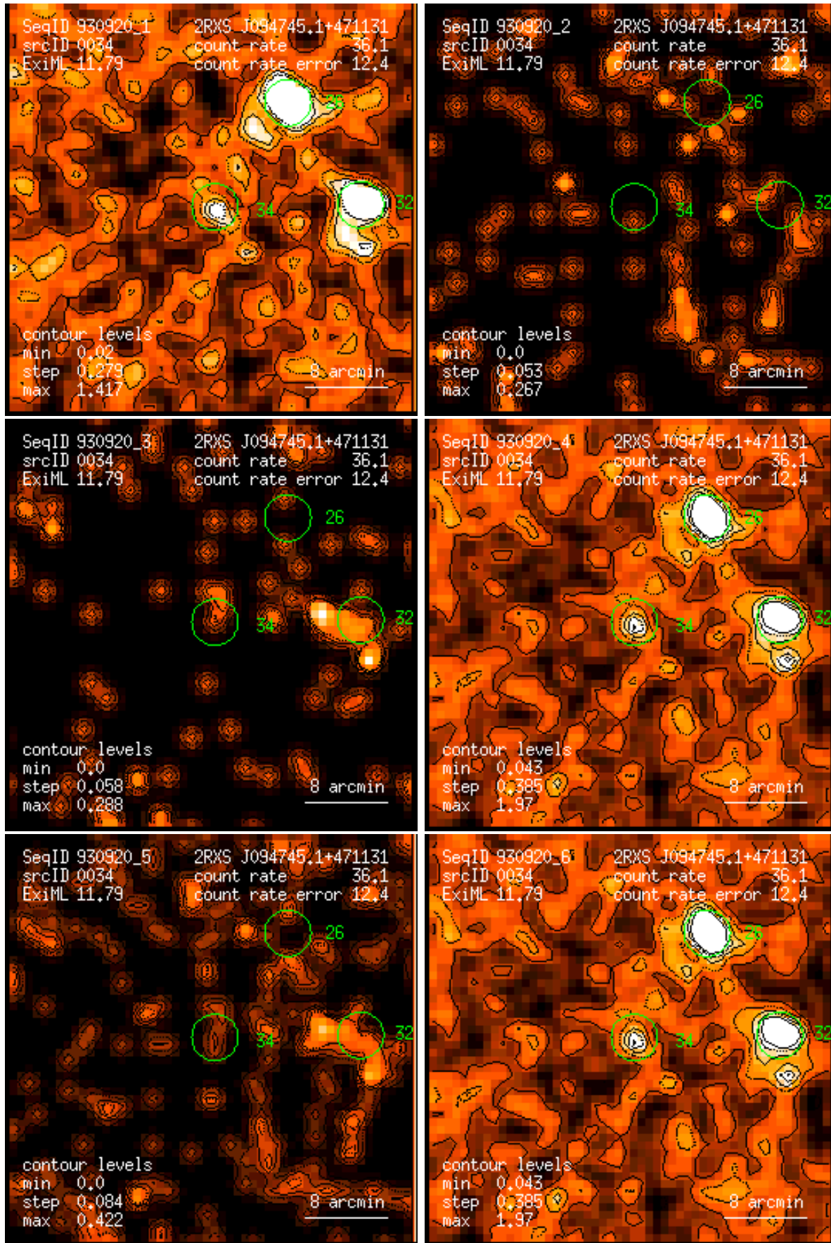
Figure 34: RASS 930920: detection 0034: band rate images, Gaussian filter: (1) PSPC channels 11 – 41, (2) 52 – 90, (3) 91 – 201, (4) 11 – 235, (5) 52 – 201, (6) 11 – 201. Broad band rates in counts/ks. Band rate contour levels in counts/ks/arcmin 2 .
