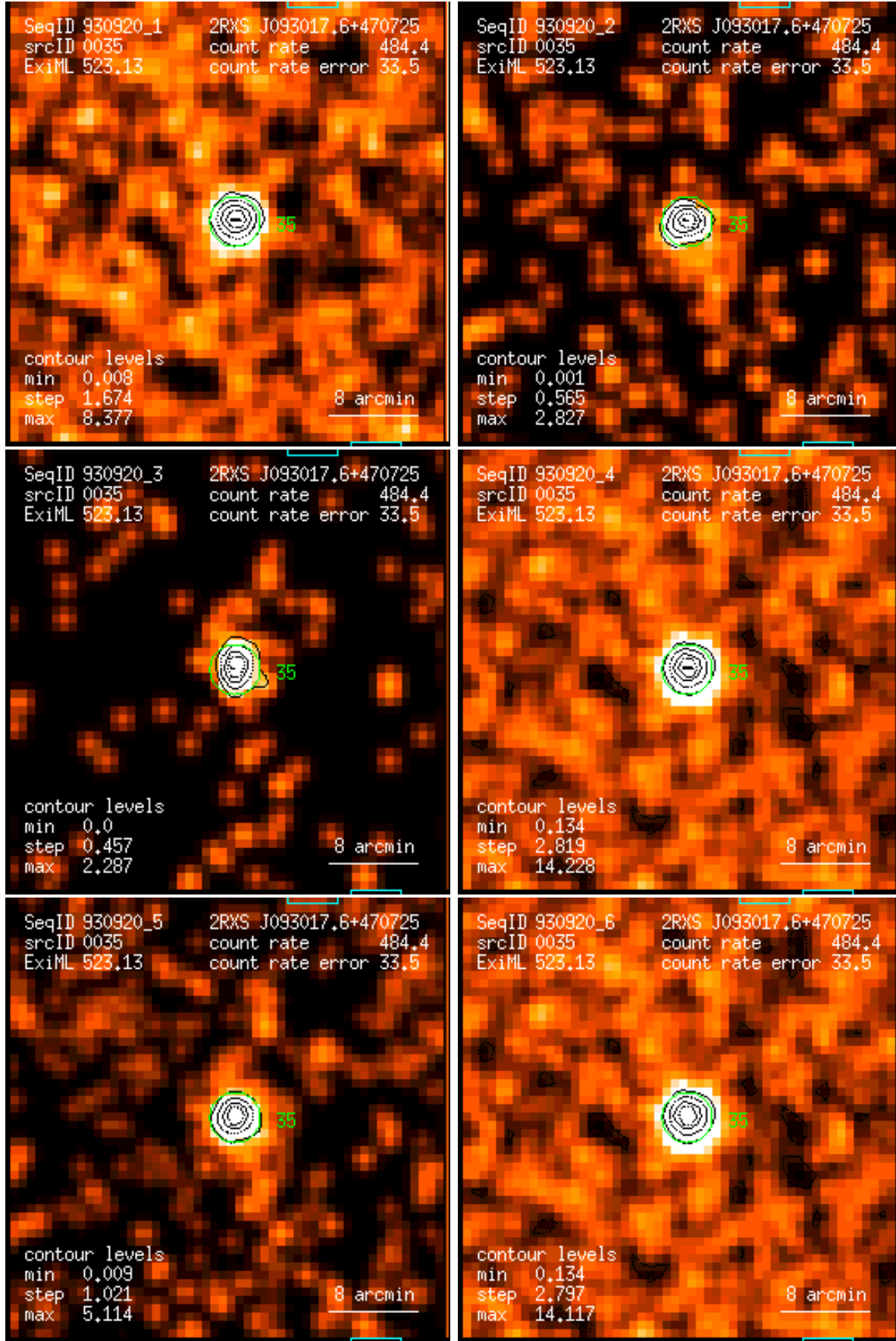
Figure 35: RASS 930920: detection 0035: band rate images, Gaussian filter: (1) PSPC channels 11 – 41, (2) 52 – 90, (3) 91 – 201, (4) 11 – 235, (5) 52 – 201, (6) 11 – 201. Broad band rates in counts/ks. Band rate contour levels in counts/ks/arcmin 2 .
