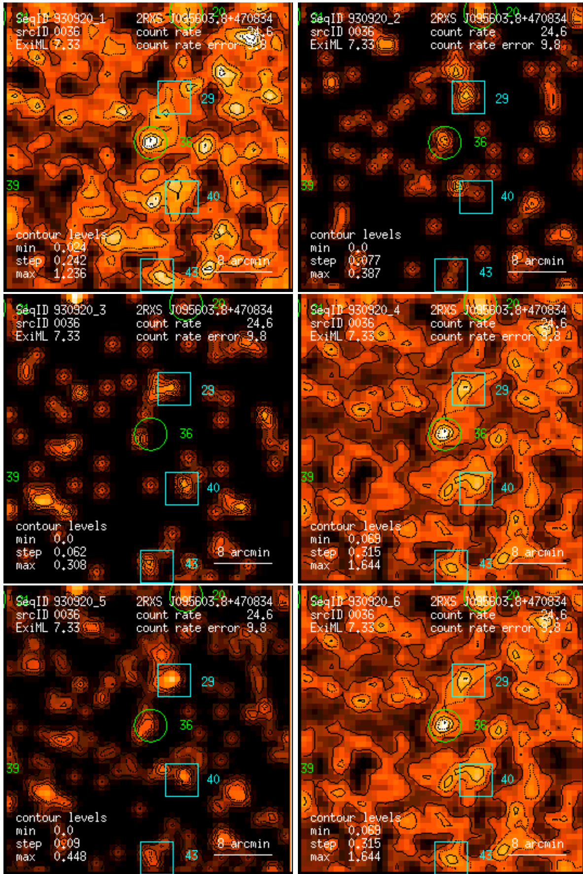
Figure 36: RASS 930920: detection 0036: band rate images, Gaussian filter: (1) PSPC channels 11 – 41, (2) 52 – 90, (3) 91 – 201, (4) 11 – 235, (5) 52 – 201, (6) 11 – 201. Broad band rates in counts/ks. Band rate contour levels in counts/ks/arcmin 2 .
