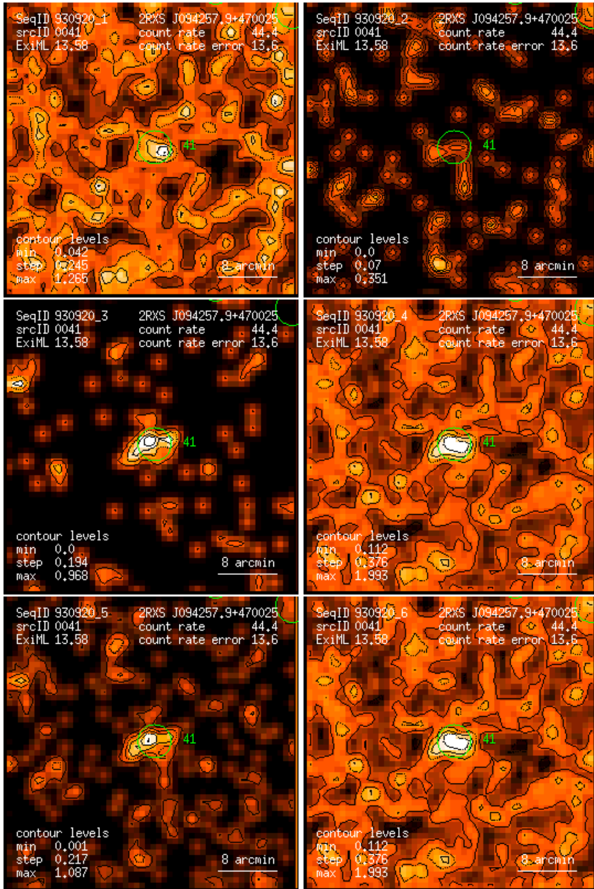
Figure 41: RASS 930920: detection 0041: band rate images, Gaussian filter: (1) PSPC channels 11 – 41, (2) 52 – 90, (3) 91 – 201, (4) 11 – 235, (5) 52 – 201, (6) 11 – 201. Broad band rates in counts/ks. Band rate contour levels in counts/ks/arcmin 2 .
