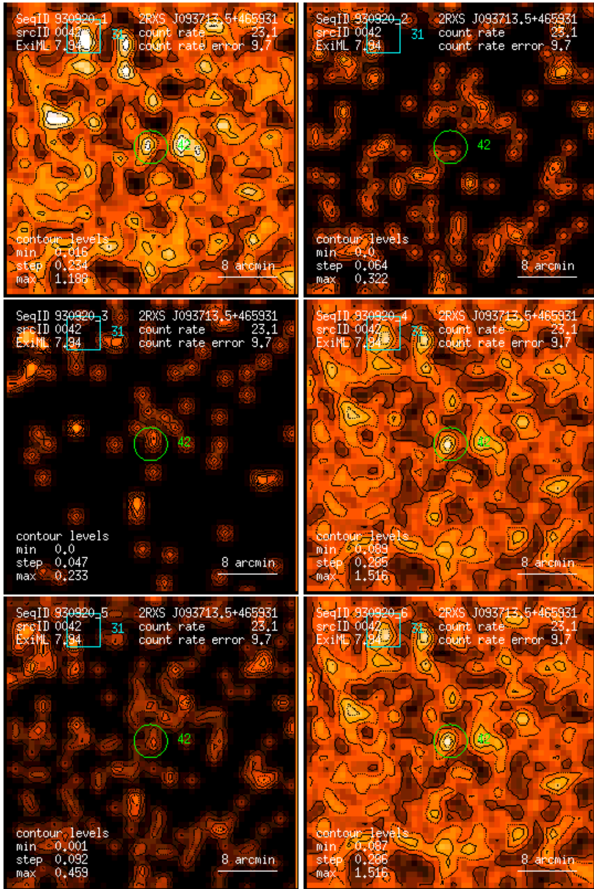
Figure 42: RASS 930920: detection 0042: band rate images, Gaussian filter: (1) PSPC channels 11 – 41, (2) 52 – 90, (3) 91 – 201, (4) 11 – 235, (5) 52 – 201, (6) 11 – 201. Broad band rates in counts/ks. Band rate contour levels in counts/ks/arcmin 2 .
