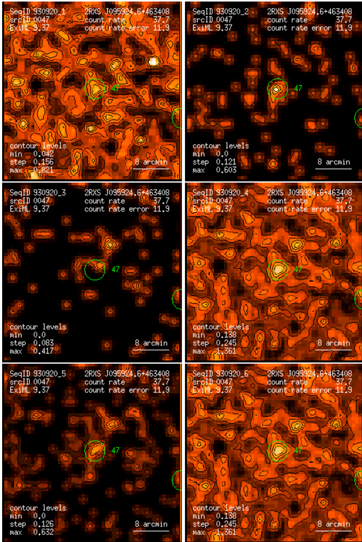
Figure 47: RASS 930920: detection 0047: band rate images, Gaussian filter: (1) PSPC channels 11 – 41, (2) 52 – 90, (3) 91 – 201, (4) 11 – 235, (5) 52 – 201, (6) 11 – 201. Broad band rates in counts/ks. Band rate contour levels in counts/ks/arcmin 2 .
