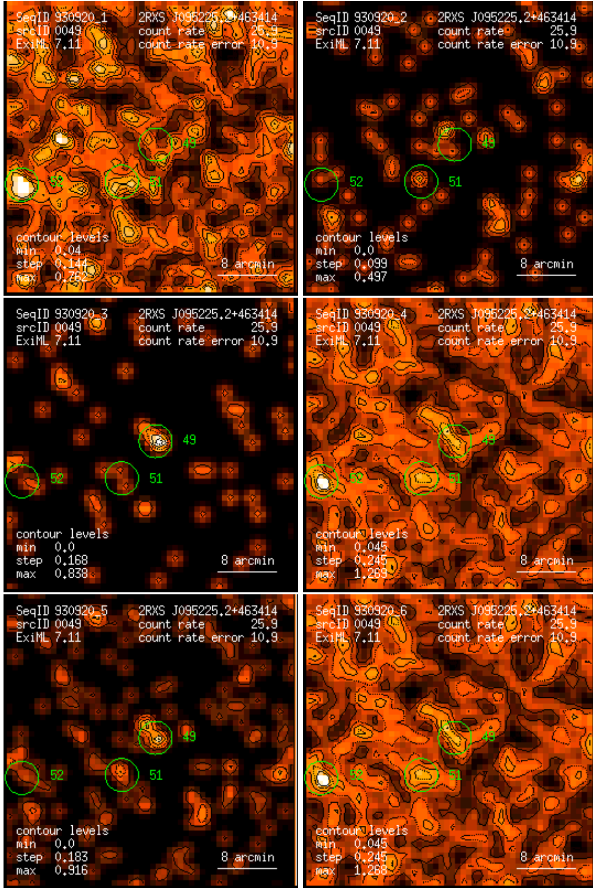
Figure 49: RASS 930920: detection 0049: band rate images, Gaussian filter: (1) PSPC channels 11 – 41, (2) 52 – 90, (3) 91 – 201, (4) 11 – 235, (5) 52 – 201, (6) 11 – 201. Broad band rates in counts/ks. Band rate contour levels in counts/ks/arcmin 2 .
