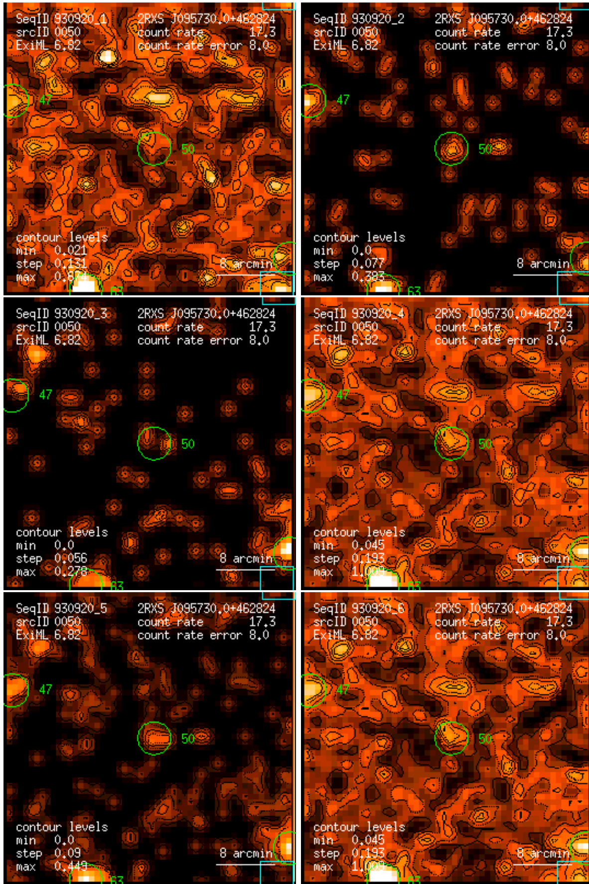
Figure 50: RASS 930920: detection 0050: band rate images, Gaussian filter: (1) PSPC channels 11 – 41, (2) 52 – 90, (3) 91 – 201, (4) 11 – 235, (5) 52 – 201, (6) 11 – 201. Broad band rates in counts/ks. Band rate contour levels in counts/ks/arcmin 2 .
