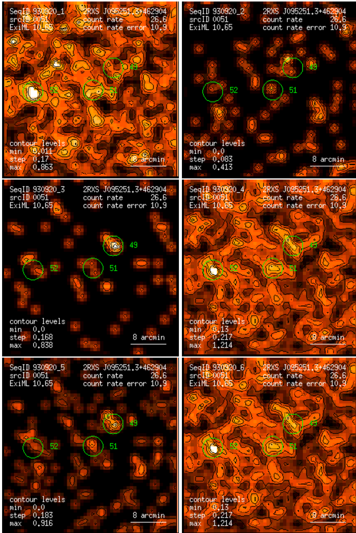
Figure 51: RASS 930920: detection 0051: band rate images, Gaussian filter: (1) PSPC channels 11 – 41, (2) 52 – 90, (3) 91 – 201, (4) 11 – 235, (5) 52 – 201, (6) 11 – 201. Broad band rates in counts/ks. Band rate contour levels in counts/ks/arcmin 2 .
