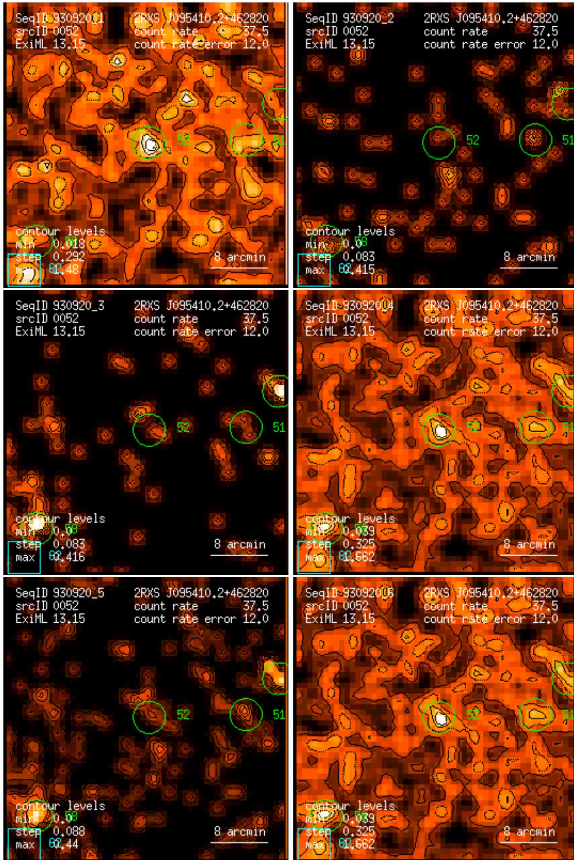
Figure 52: RASS 930920: detection 0052: band rate images, Gaussian filter: (1) PSPC channels 11 – 41, (2) 52 – 90, (3) 91 – 201, (4) 11 – 235, (5) 52 – 201, (6) 11 – 201. Broad band rates in counts/ks. Band rate contour levels in counts/ks/arcmin 2 .
