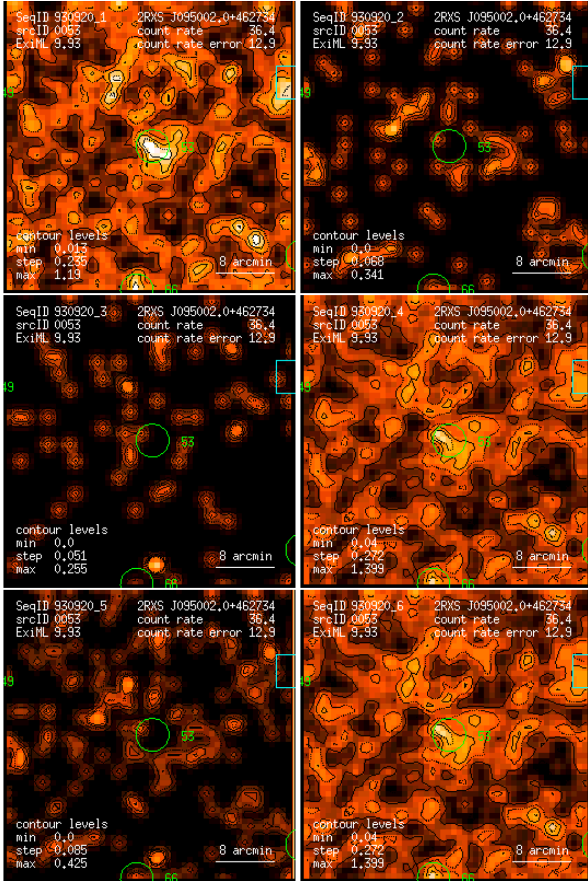
Figure 53: RASS 930920: detection 0053: band rate images, Gaussian filter: (1) PSPC channels 11 – 41, (2) 52 – 90, (3) 91 – 201, (4) 11 – 235, (5) 52 – 201, (6) 11 – 201. Broad band rates in counts/ks. Band rate contour levels in counts/ks/arcmin 2 .
