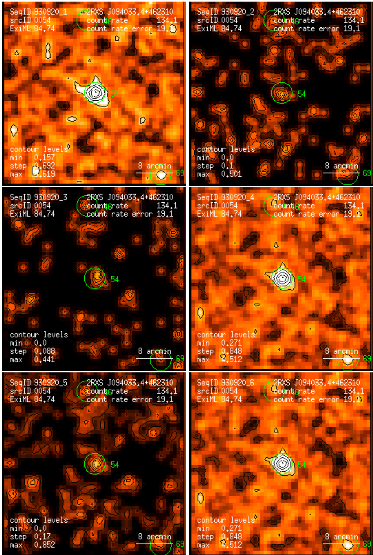
Figure 54: RASS 930920: detection 0054: band rate images, Gaussian filter: (1) PSPC channels 11 – 41, (2) 52 – 90, (3) 91 – 201, (4) 11 – 235, (5) 52 – 201, (6) 11 – 201. Broad band rates in counts/ks. Band rate contour levels in counts/ks/arcmin 2 .
