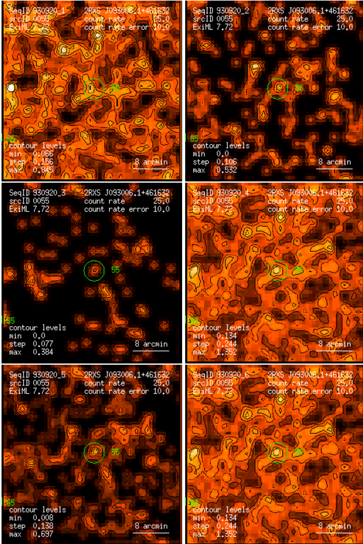
Figure 55: RASS 930920: detection 0055: band rate images, Gaussian filter: (1) PSPC channels 11 – 41, (2) 52 – 90, (3) 91 – 201, (4) 11 – 235, (5) 52 – 201, (6) 11 – 201. Broad band rates in counts/ks. Band rate contour levels in counts/ks/arcmin 2 .
