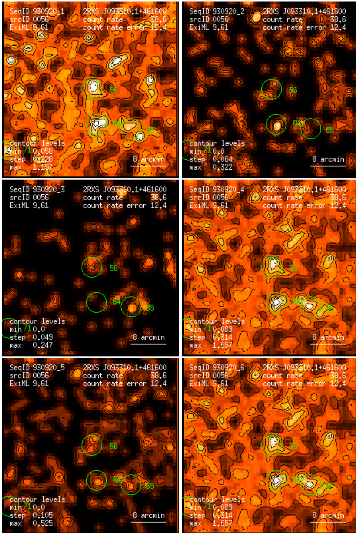
Figure 56: RASS 930920: detection 0056: band rate images, Gaussian filter: (1) PSPC channels 11 – 41, (2) 52 – 90, (3) 91 – 201, (4) 11 – 235, (5) 52 – 201, (6) 11 – 201. Broad band rates in counts/ks. Band rate contour levels in counts/ks/arcmin 2 .
