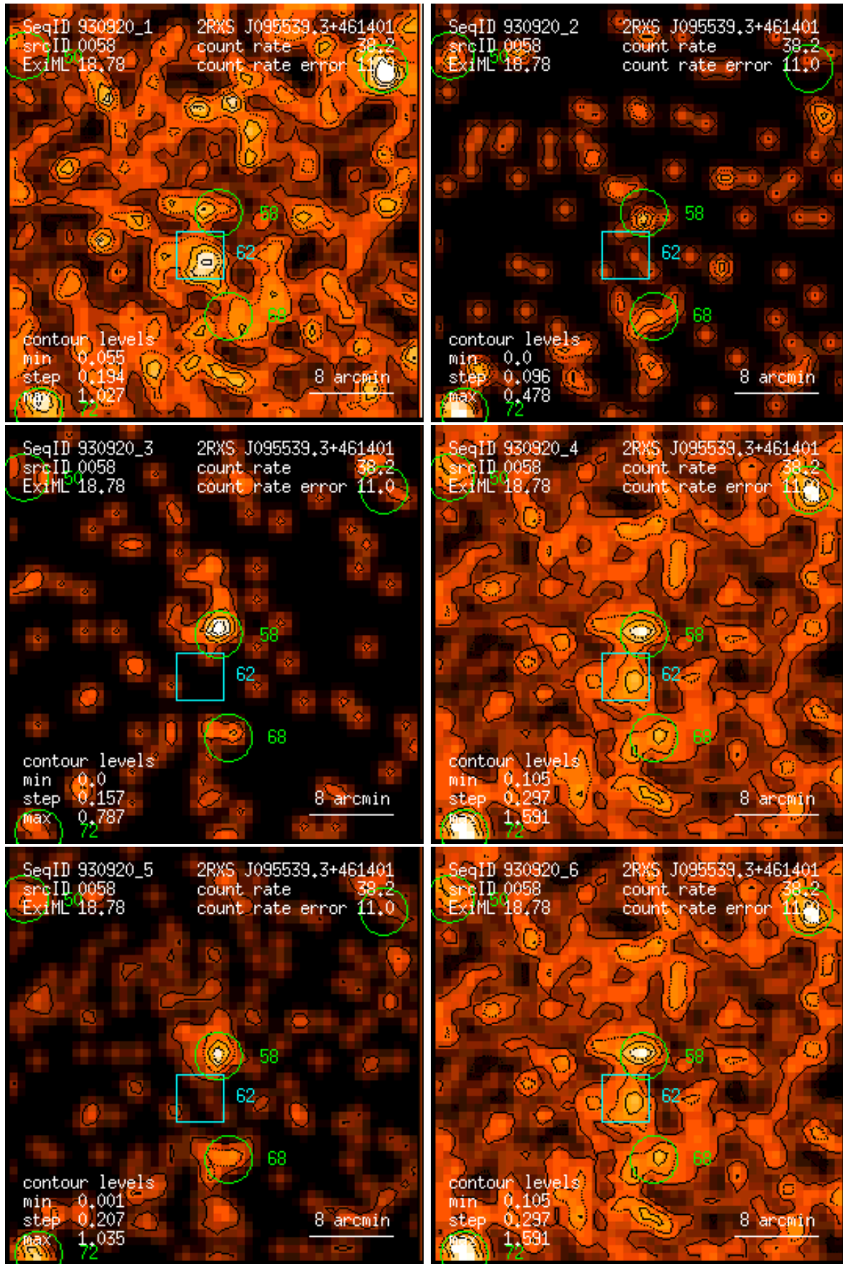
Figure 58: RASS 930920: detection 0058: band rate images, Gaussian filter: (1) PSPC channels 11 – 41, (2) 52 – 90, (3) 91 – 201, (4) 11 – 235, (5) 52 – 201, (6) 11 – 201. Broad band rates in counts/ks. Band rate contour levels in counts/ks/arcmin 2 .
