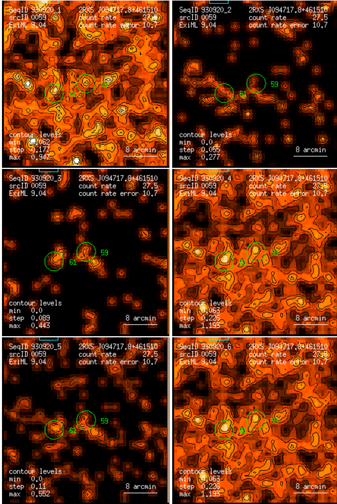
Figure 59: RASS 930920: detection 0059: band rate images, Gaussian filter: (1) PSPC channels 11 – 41, (2) 52 – 90, (3) 91 – 201, (4) 11 – 235, (5) 52 – 201, (6) 11 – 201. Broad band rates in counts/ks. Band rate contour levels in counts/ks/arcmin 2 .
