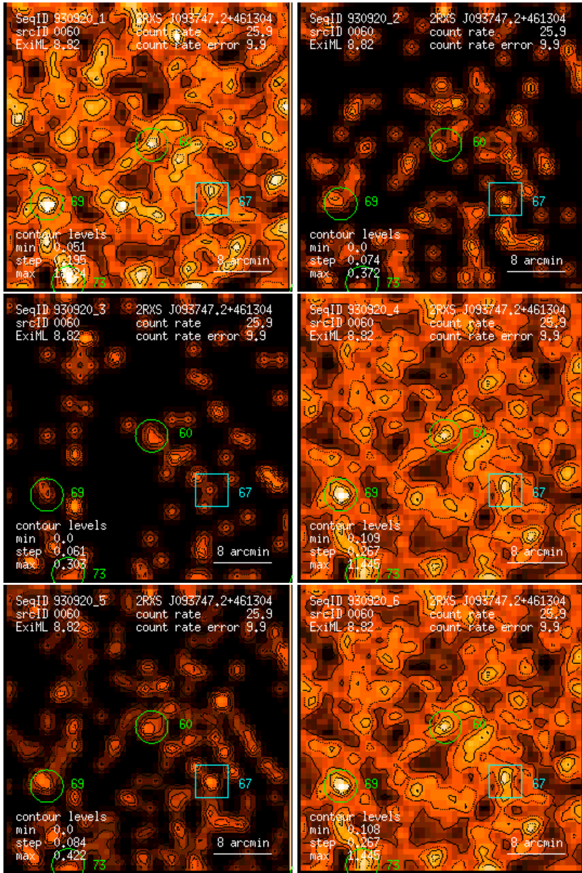
Figure 60: RASS 930920: detection 0060: band rate images, Gaussian filter: (1) PSPC channels 11 – 41, (2) 52 – 90, (3) 91 – 201, (4) 11 – 235, (5) 52 – 201, (6) 11 – 201. Broad band rates in counts/ks. Band rate contour levels in counts/ks/arcmin 2 .
