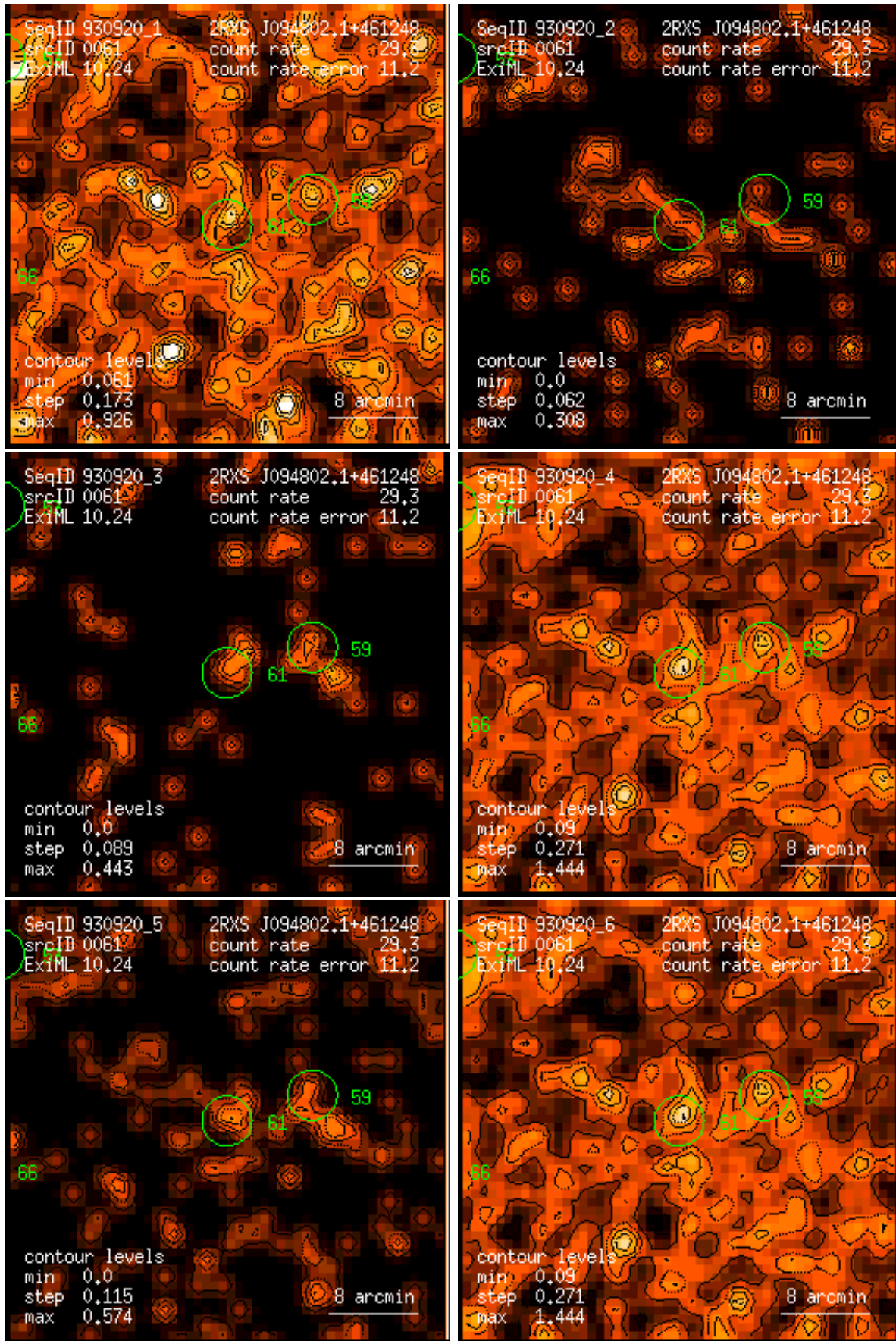
Figure 61: RASS 930920: detection 0061: band rate images, Gaussian filter: (1) PSPC channels 11 – 41, (2) 52 – 90, (3) 91 – 201, (4) 11 – 235, (5) 52 – 201, (6) 11 – 201. Broad band rates in counts/ks. Band rate contour levels in counts/ks/arcmin 2 .
