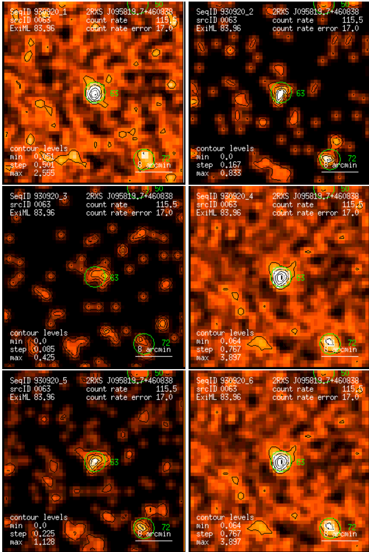
Figure 63: RASS 930920: detection 0063: band rate images, Gaussian filter: (1) PSPC channels 11 – 41, (2) 52 – 90, (3) 91 – 201, (4) 11 – 235, (5) 52 – 201, (6) 11 – 201. Broad band rates in counts/ks. Band rate contour levels in counts/ks/arcmin 2 .
