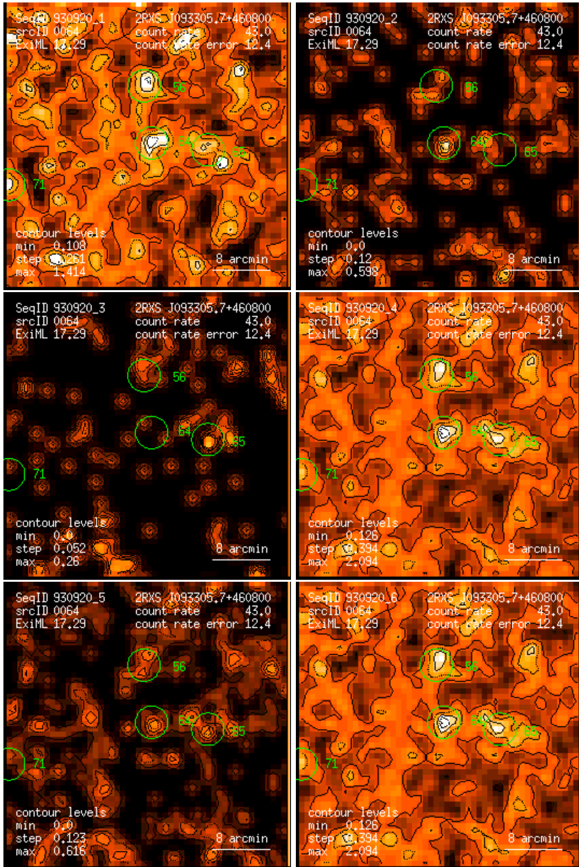
Figure 64: RASS 930920: detection 0064: band rate images, Gaussian filter: (1) PSPC channels 11 – 41, (2) 52 – 90, (3) 91 – 201, (4) 11 – 235, (5) 52 – 201, (6) 11 – 201. Broad band rates in counts/ks. Band rate contour levels in counts/ks/arcmin 2 .
