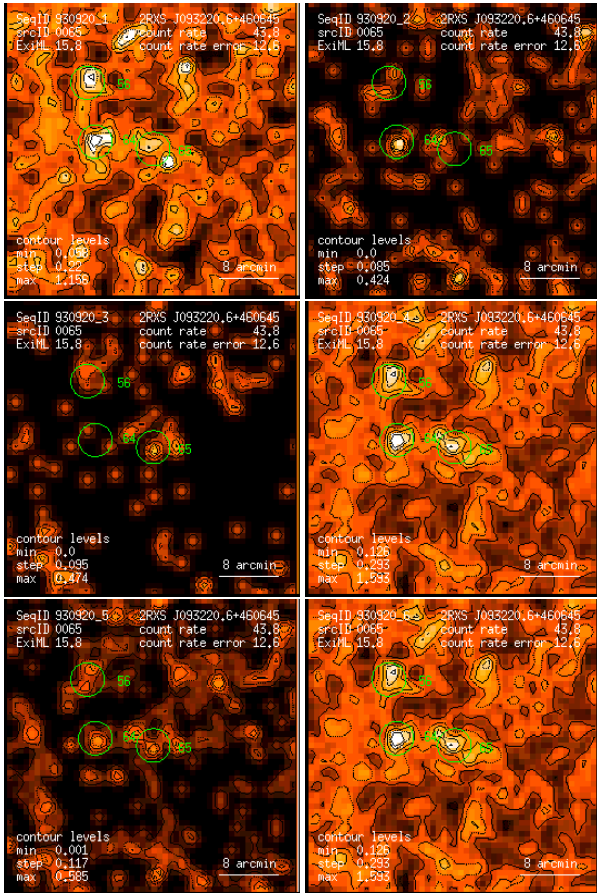
Figure 65: RASS 930920: detection 0065: band rate images, Gaussian filter: (1) PSPC channels 11 – 41, (2) 52 – 90, (3) 91 – 201, (4) 11 – 235, (5) 52 – 201, (6) 11 – 201. Broad band rates in counts/ks. Band rate contour levels in counts/ks/arcmin 2 .
