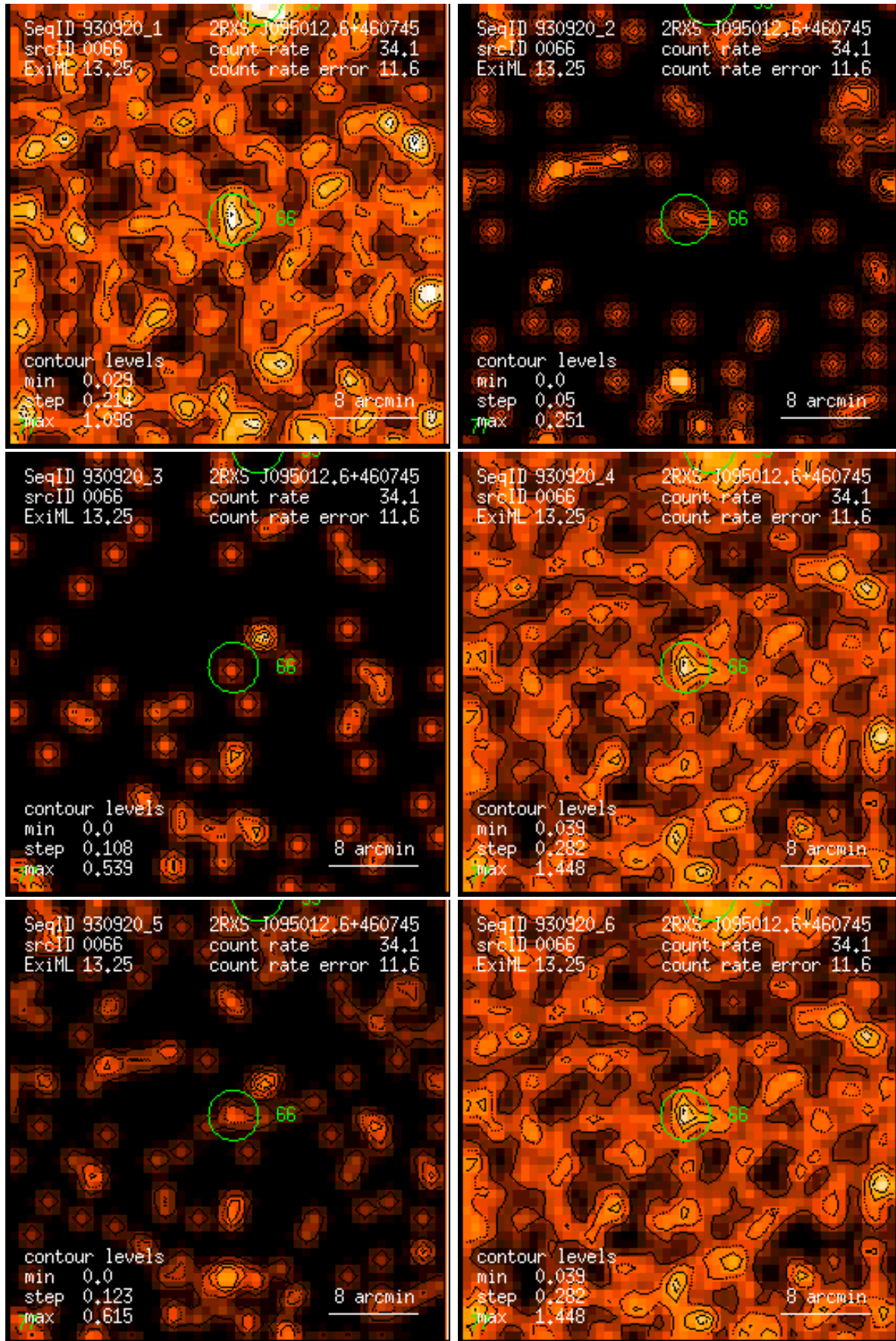
Figure 66: RASS 930920: detection 0066: band rate images, Gaussian filter: (1) PSPC channels 11 – 41, (2) 52 – 90, (3) 91 – 201, (4) 11 – 235, (5) 52 – 201, (6) 11 – 201. Broad band rates in counts/ks. Band rate contour levels in counts/ks/arcmin 2 .
