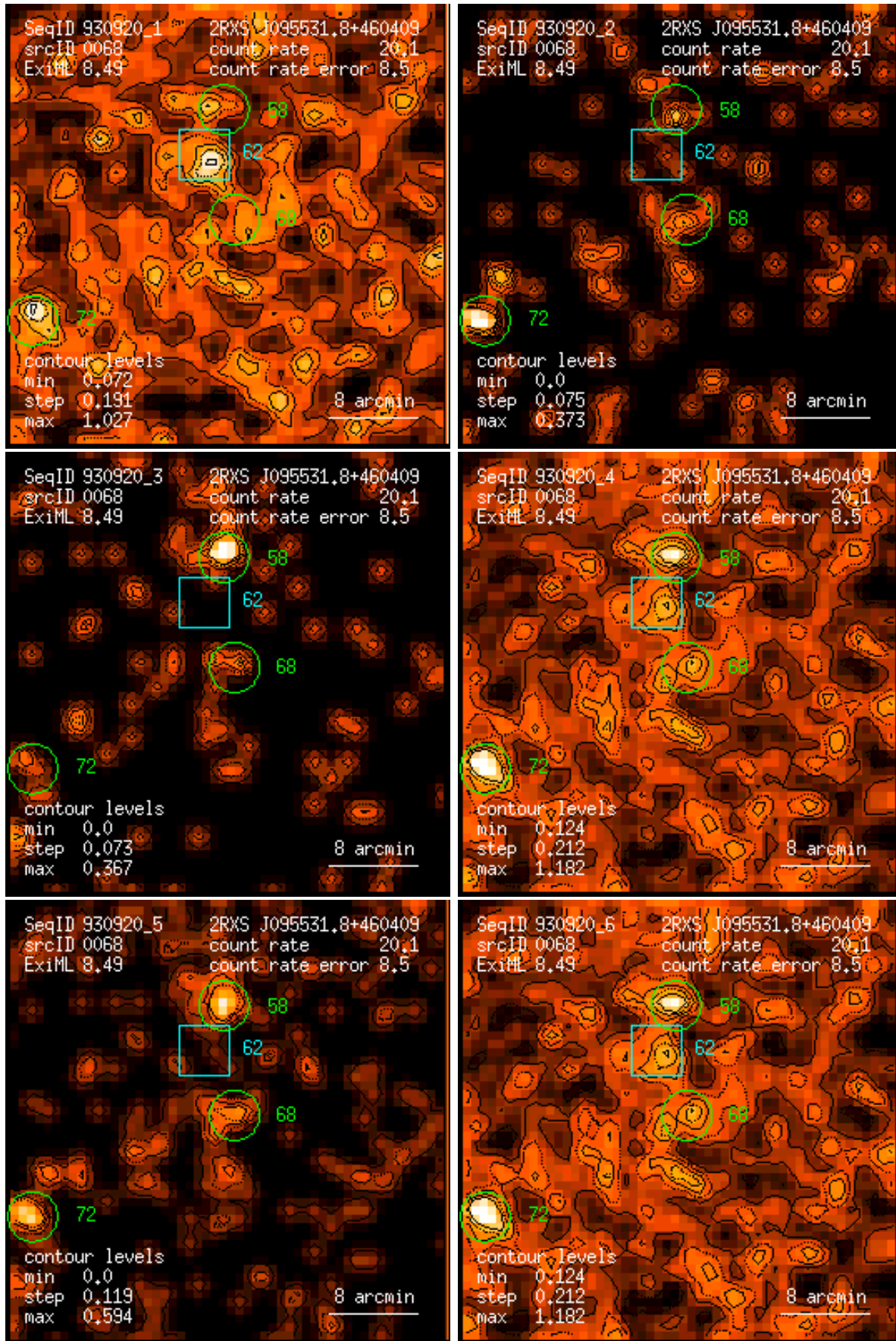
Figure 68: RASS 930920: detection 0068: band rate images, Gaussian filter: (1) PSPC channels 11 – 41, (2) 52 – 90, (3) 91 – 201, (4) 11 – 235, (5) 52 – 201, (6) 11 – 201. Broad band rates in counts/ks. Band rate contour levels in counts/ks/arcmin 2 .
