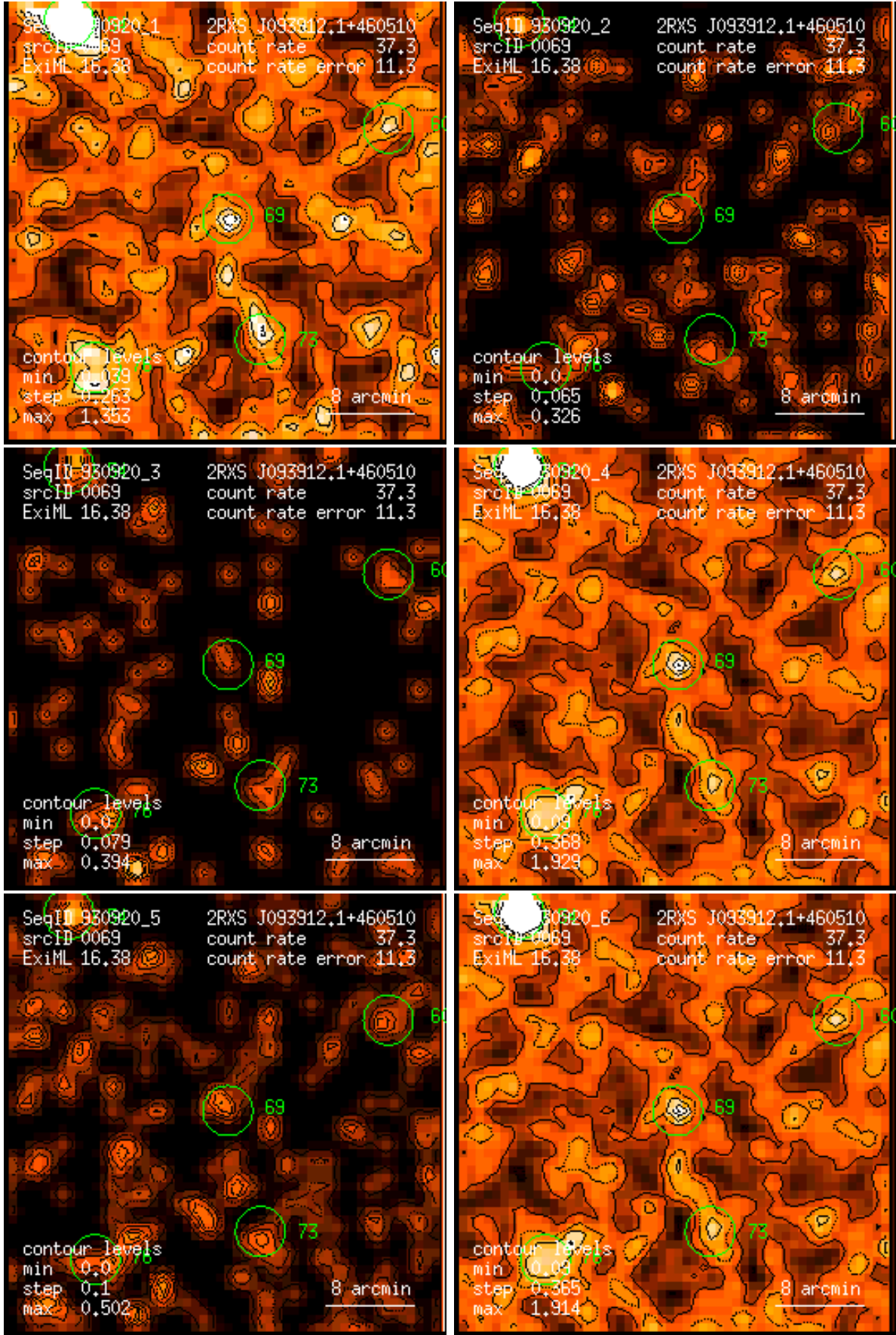
Figure 69: RASS 930920: detection 0069: band rate images, Gaussian filter: (1) PSPC channels 11 – 41, (2) 52 – 90, (3) 91 – 201, (4) 11 – 235, (5) 52 – 201, (6) 11 – 201. Broad band rates in counts/ks. Band rate contour levels in counts/ks/arcmin 2 .
