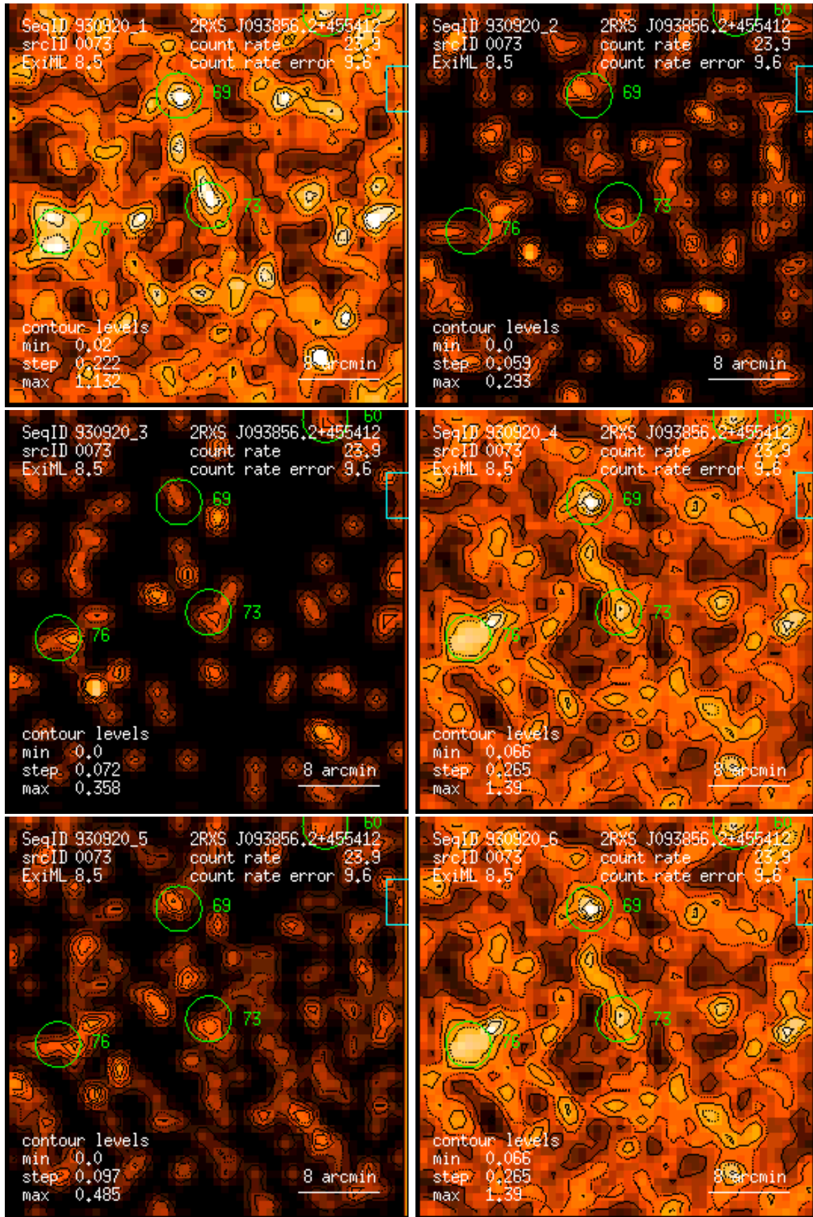
Figure 73: RASS 930920: detection 0073: band rate images, Gaussian filter: (1) PSPC channels 11 – 41, (2) 52 – 90, (3) 91 – 201, (4) 11 – 235, (5) 52 – 201, (6) 11 – 201. Broad band rates in counts/ks. Band rate contour levels in counts/ks/arcmin 2 .
