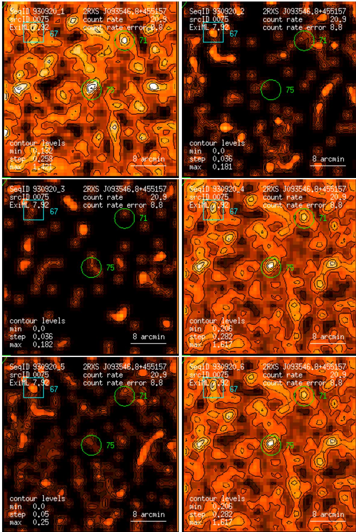
Figure 75: RASS 930920: detection 0075: band rate images, Gaussian filter: (1) PSPC channels 11 – 41, (2) 52 – 90, (3) 91 – 201, (4) 11 – 235, (5) 52 – 201, (6) 11 – 201. Broad band rates in counts/ks. Band rate contour levels in counts/ks/arcmin 2 .
