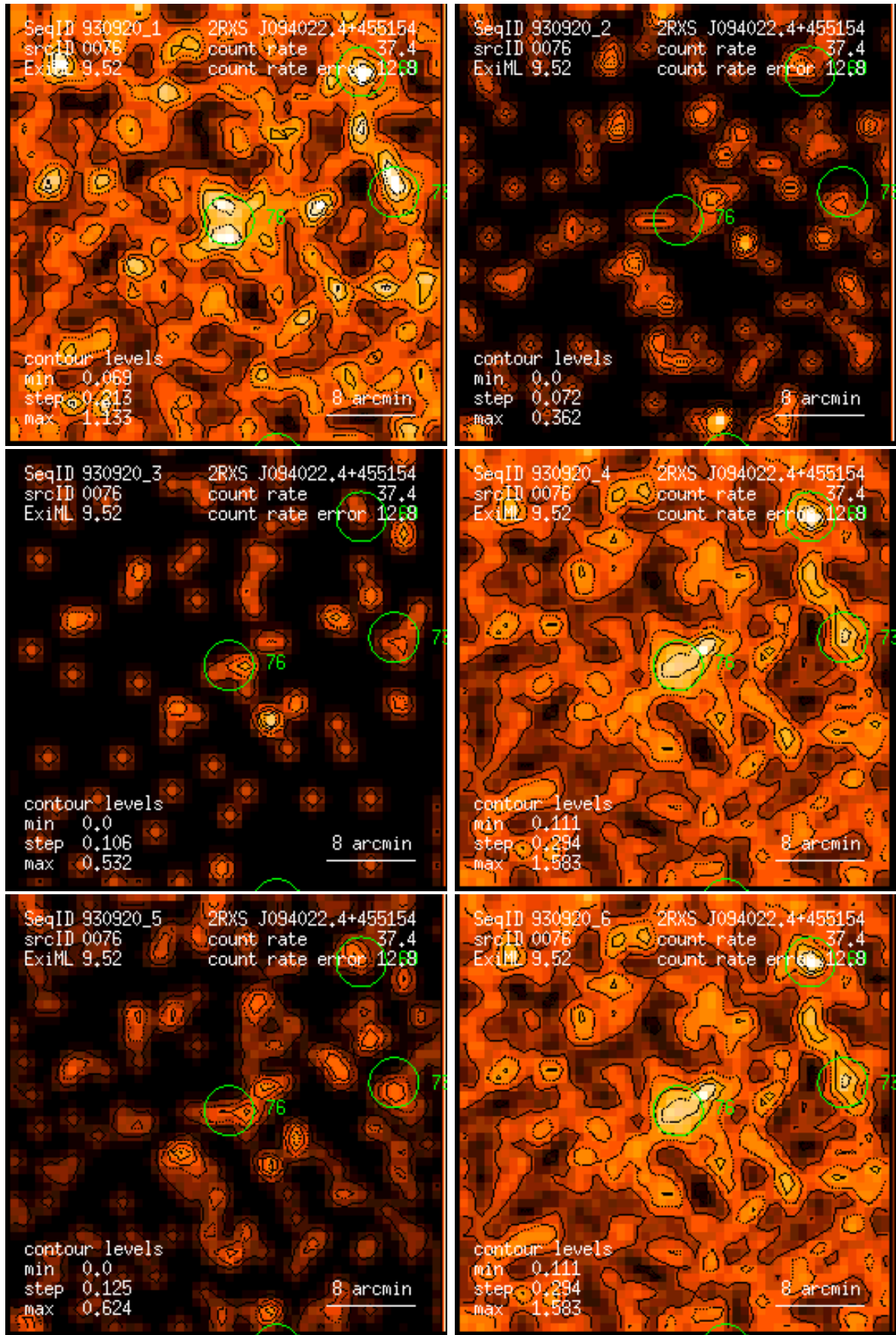
Figure 76: RASS 930920: detection 0076: band rate images, Gaussian filter: (1) PSPC channels 11 – 41, (2) 52 – 90, (3) 91 – 201, (4) 11 – 235, (5) 52 – 201, (6) 11 – 201. Broad band rates in counts/ks. Band rate contour levels in counts/ks/arcmin 2 .
