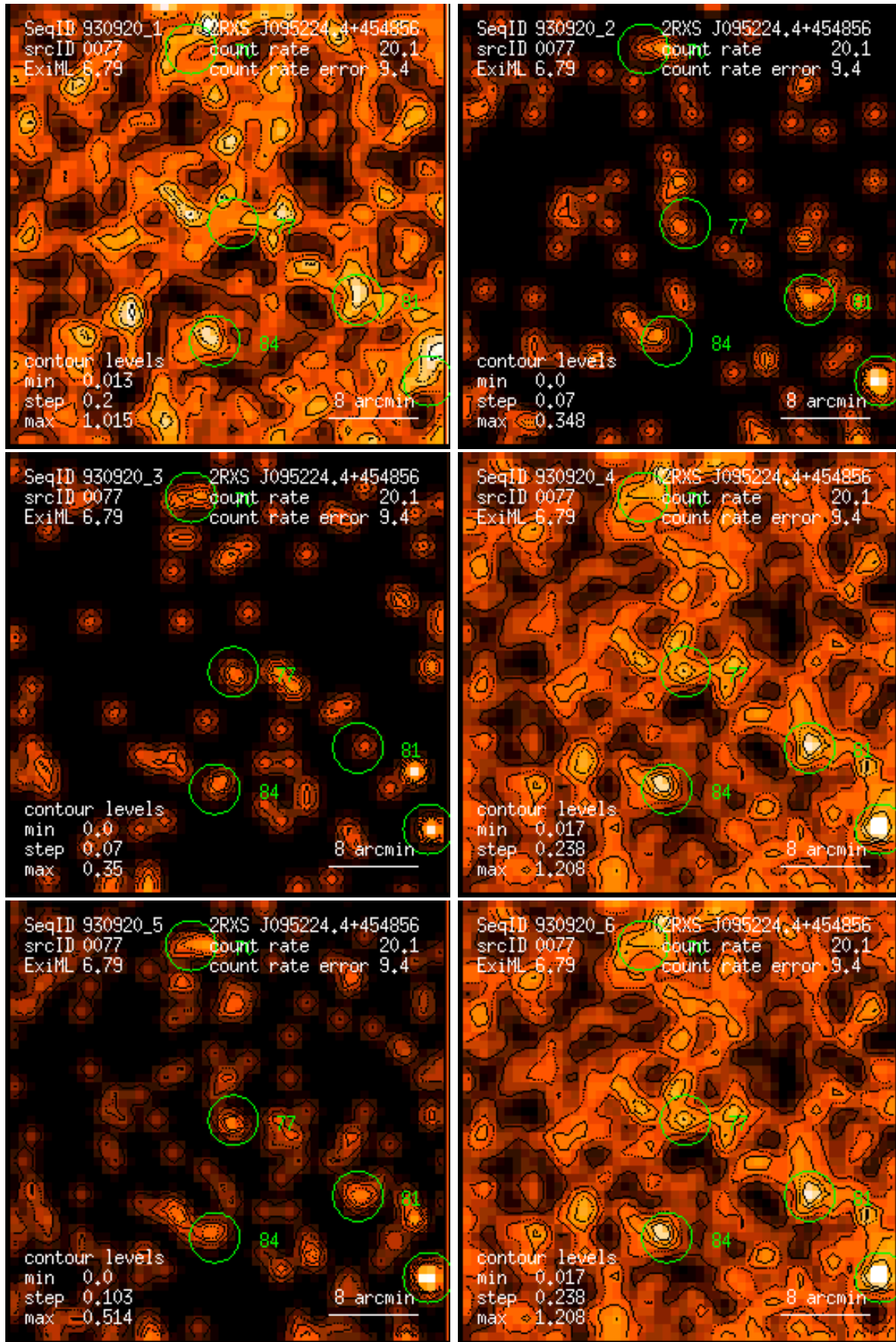
Figure 77: RASS 930920: detection 0077: band rate images, Gaussian filter: (1) PSPC channels 11 – 41, (2) 52 – 90, (3) 91 – 201, (4) 11 – 235, (5) 52 – 201, (6) 11 – 201. Broad band rates in counts/ks. Band rate contour levels in counts/ks/arcmin 2 .
