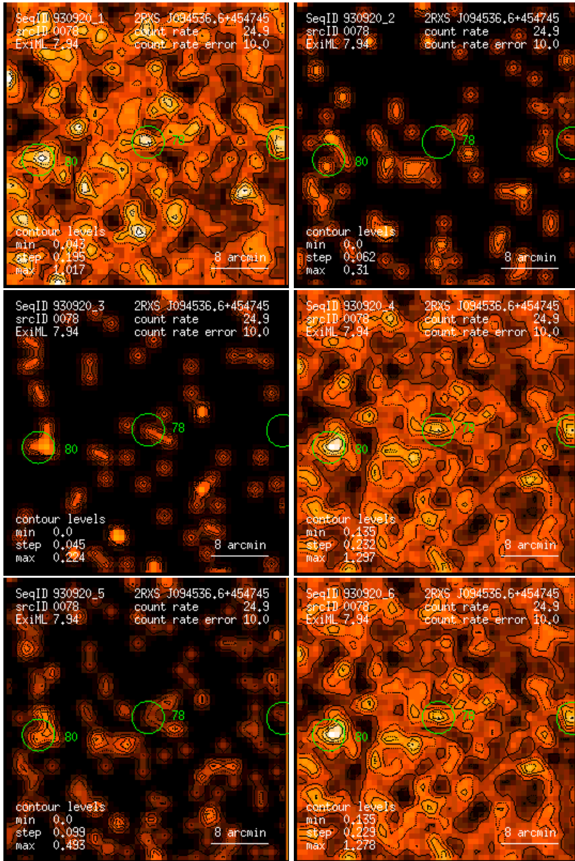
Figure 78: RASS 930920: detection 0078: band rate images, Gaussian filter: (1) PSPC channels 11 – 41, (2) 52 – 90, (3) 91 – 201, (4) 11 – 235, (5) 52 – 201, (6) 11 – 201. Broad band rates in counts/ks. Band rate contour levels in counts/ks/arcmin 2 .
