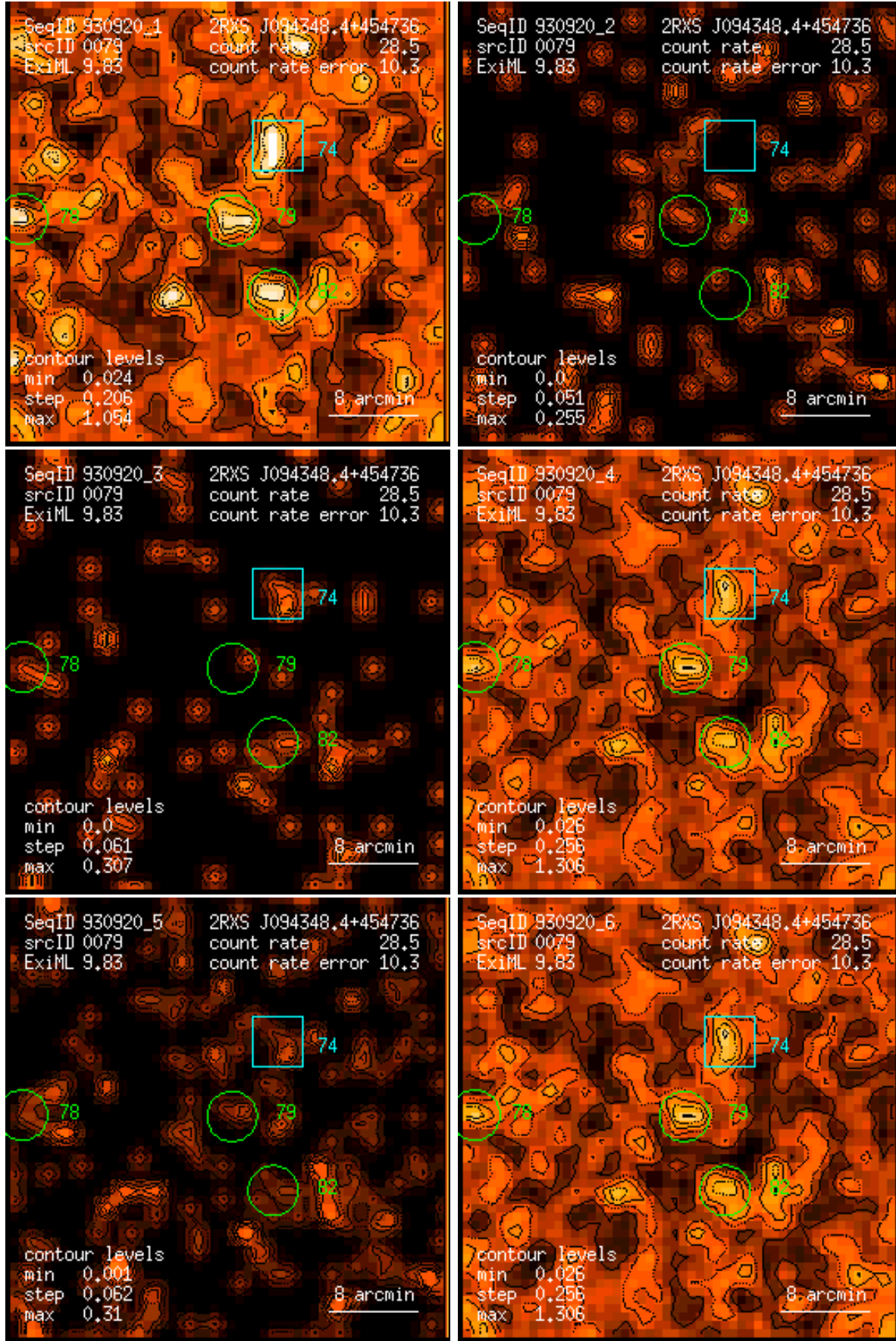
Figure 79: RASS 930920: detection 0079: band rate images, Gaussian filter: (1) PSPC channels 11 – 41, (2) 52 – 90, (3) 91 – 201, (4) 11 – 235, (5) 52 – 201, (6) 11 – 201. Broad band rates in counts/ks. Band rate contour levels in counts/ks/arcmin 2 .
