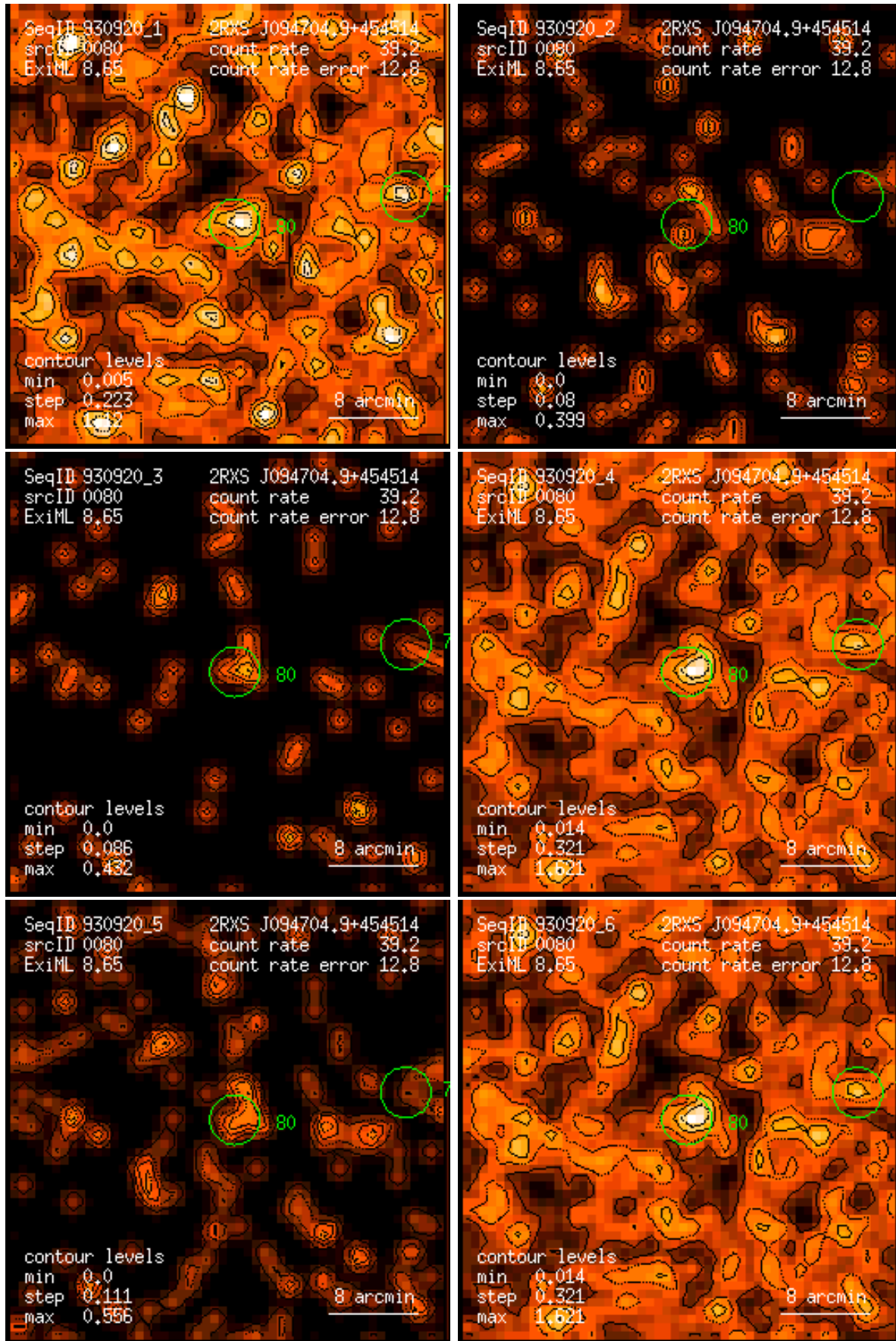
Figure 80: RASS 930920: detection 0080: band rate images, Gaussian filter: (1) PSPC channels 11 – 41, (2) 52 – 90, (3) 91 – 201, (4) 11 – 235, (5) 52 – 201, (6) 11 – 201. Broad band rates in counts/ks. Band rate contour levels in counts/ks/arcmin 2 .
