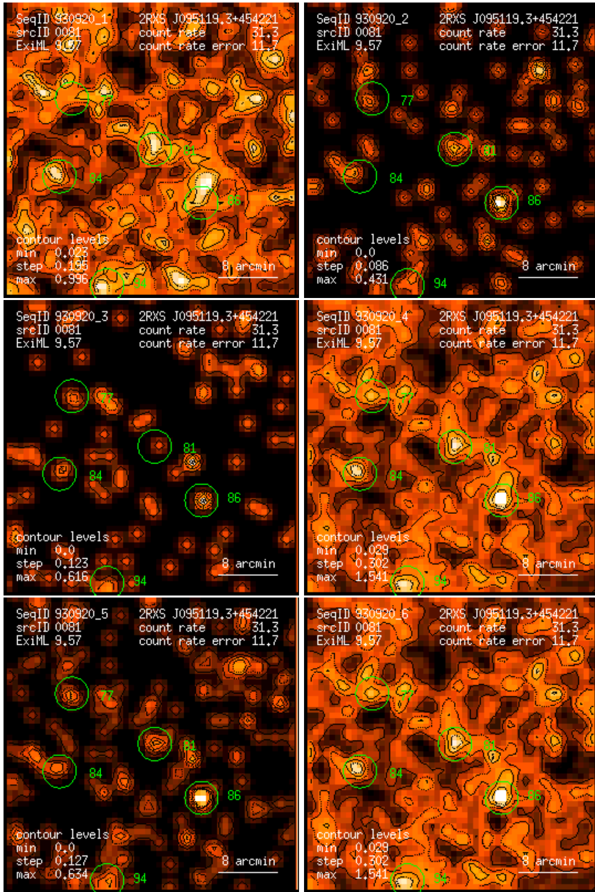
Figure 81: RASS 930920: detection 0081: band rate images, Gaussian filter: (1) PSPC channels 11 – 41, (2) 52 – 90, (3) 91 – 201, (4) 11 – 235, (5) 52 – 201, (6) 11 – 201. Broad band rates in counts/ks. Band rate contour levels in counts/ks/arcmin 2 .
