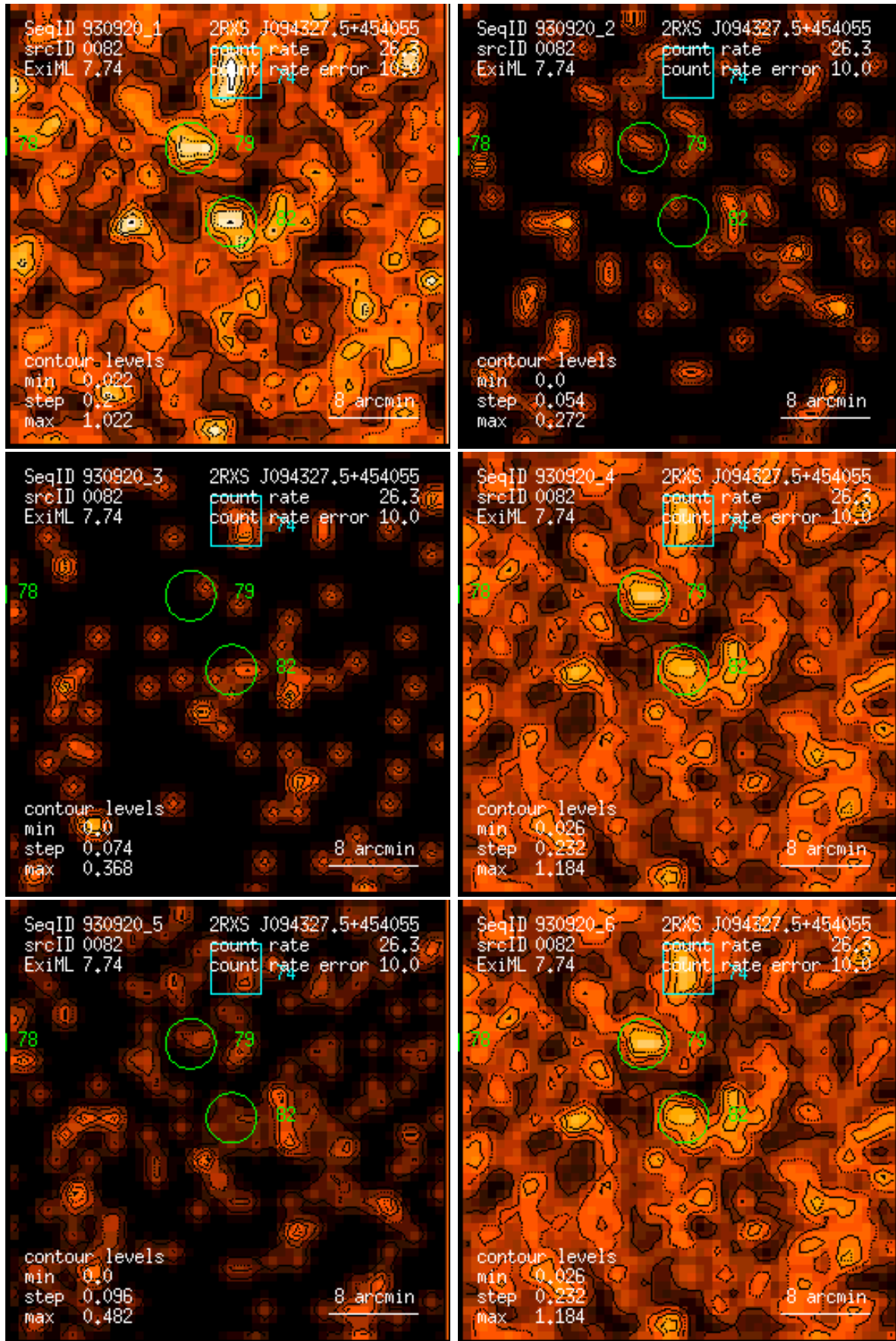
Figure 82: RASS 930920: detection 0082: band rate images, Gaussian filter: (1) PSPC channels 11 – 41, (2) 52 – 90, (3) 91 – 201, (4) 11 – 235, (5) 52 – 201, (6) 11 – 201. Broad band rates in counts/ks. Band rate contour levels in counts/ks/arcmin 2 .
