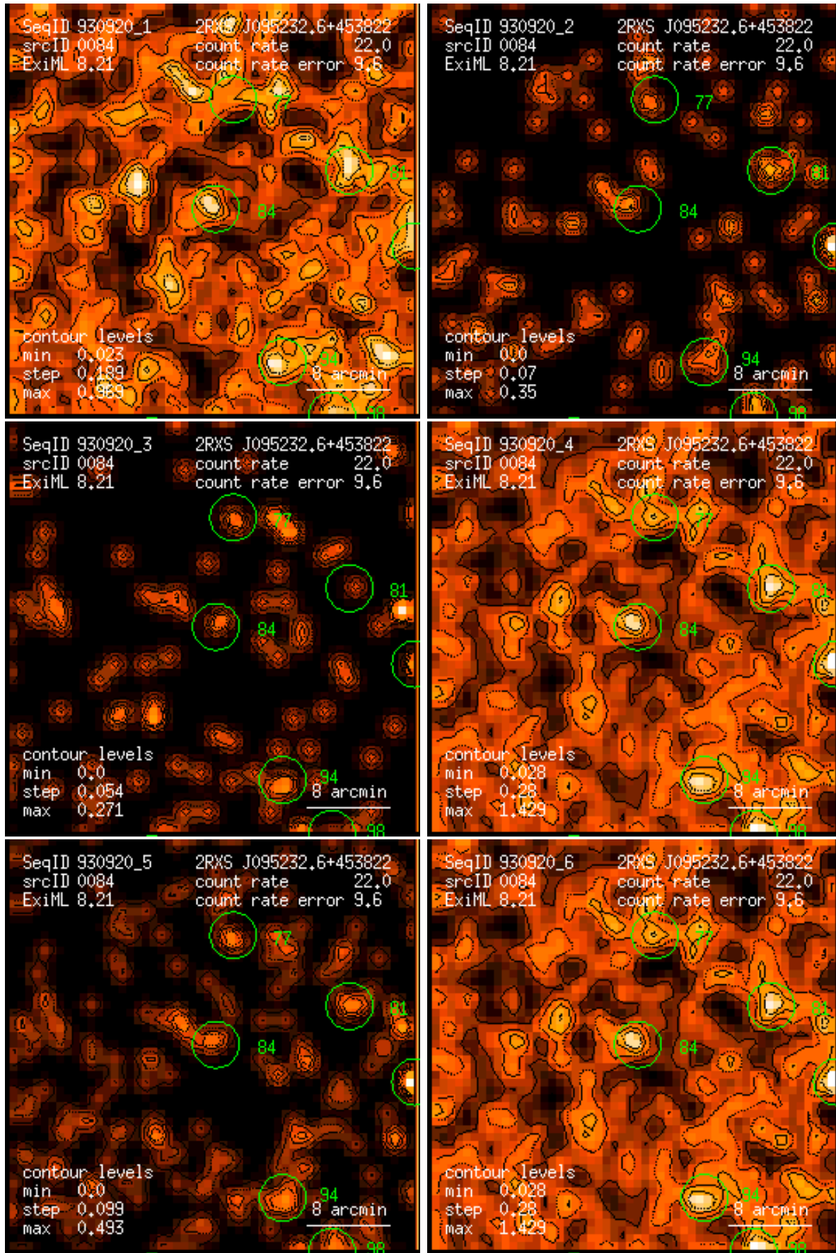
Figure 84: RASS 930920: detection 0084: band rate images, Gaussian filter: (1) PSPC channels 11 – 41, (2) 52 – 90, (3) 91 – 201, (4) 11 – 235, (5) 52 – 201, (6) 11 – 201. Broad band rates in counts/ks. Band rate contour levels in counts/ks/arcmin 2 .
