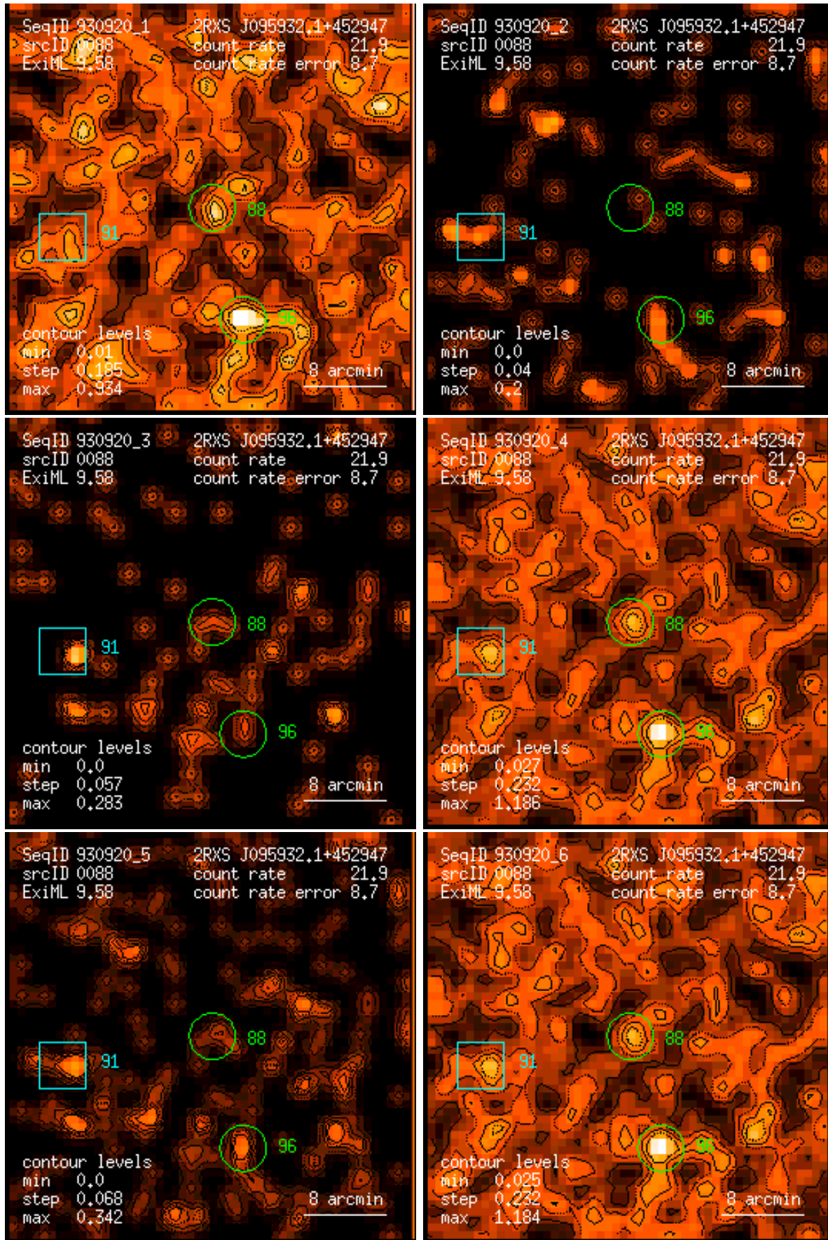
Figure 88: RASS 930920: detection 0088: band rate images, Gaussian filter: (1) PSPC channels 11 – 41, (2) 52 – 90, (3) 91 – 201, (4) 11 – 235, (5) 52 – 201, (6) 11 – 201. Broad band rates in counts/ks. Band rate contour levels in counts/ks/arcmin 2 .
