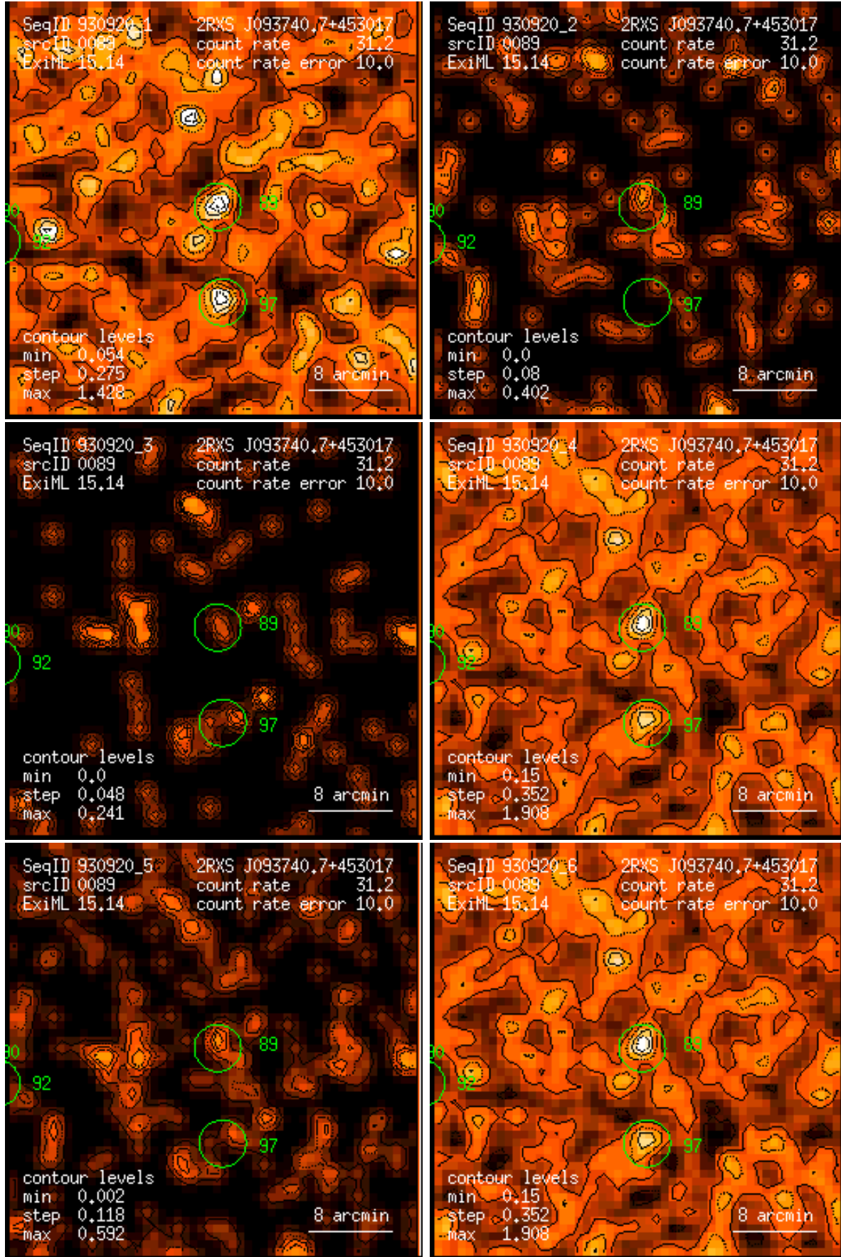
Figure 89: RASS 930920: detection 0089: band rate images, Gaussian filter: (1) PSPC channels 11 – 41, (2) 52 – 90, (3) 91 – 201, (4) 11 – 235, (5) 52 – 201, (6) 11 – 201. Broad band rates in counts/ks. Band rate contour levels in counts/ks/arcmin 2 .
