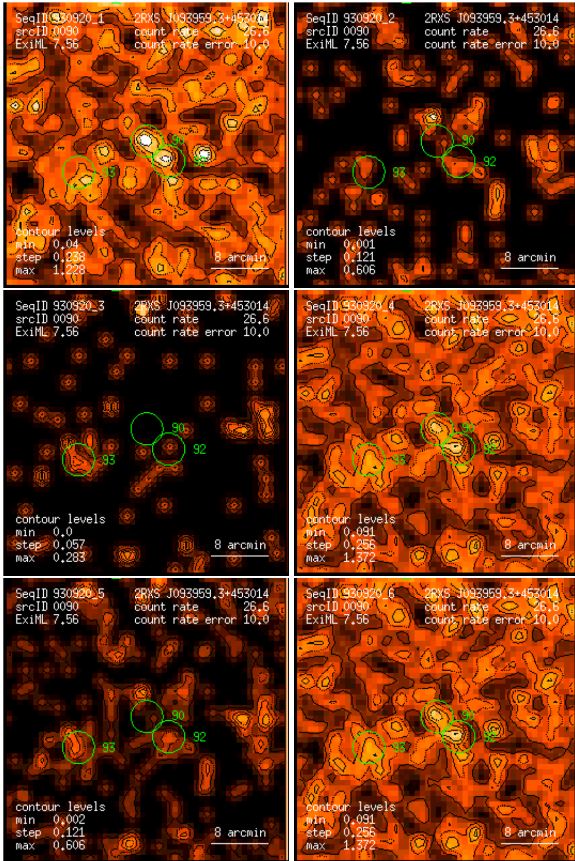
Figure 90: RASS 930920: detection 0090: band rate images, Gaussian filter: (1) PSPC channels 11 – 41, (2) 52 – 90, (3) 91 – 201, (4) 11 – 235, (5) 52 – 201, (6) 11 – 201. Broad band rates in counts/ks. Band rate contour levels in counts/ks/arcmin 2 .
