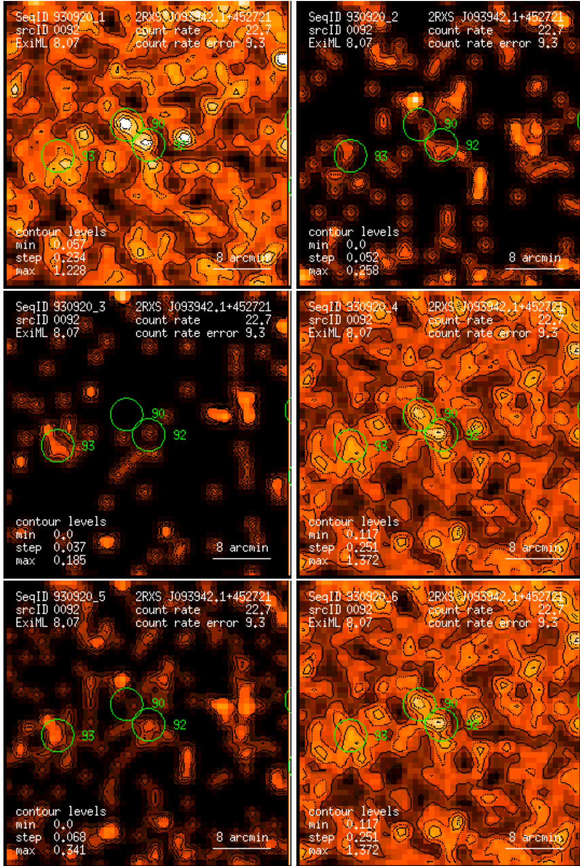
Figure 92: RASS 930920: detection 0092: band rate images, Gaussian filter: (1) PSPC channels 11 – 41, (2) 52 – 90, (3) 91 – 201, (4) 11 – 235, (5) 52 – 201, (6) 11 – 201. Broad band rates in counts/ks. Band rate contour levels in counts/ks/arcmin 2 .
