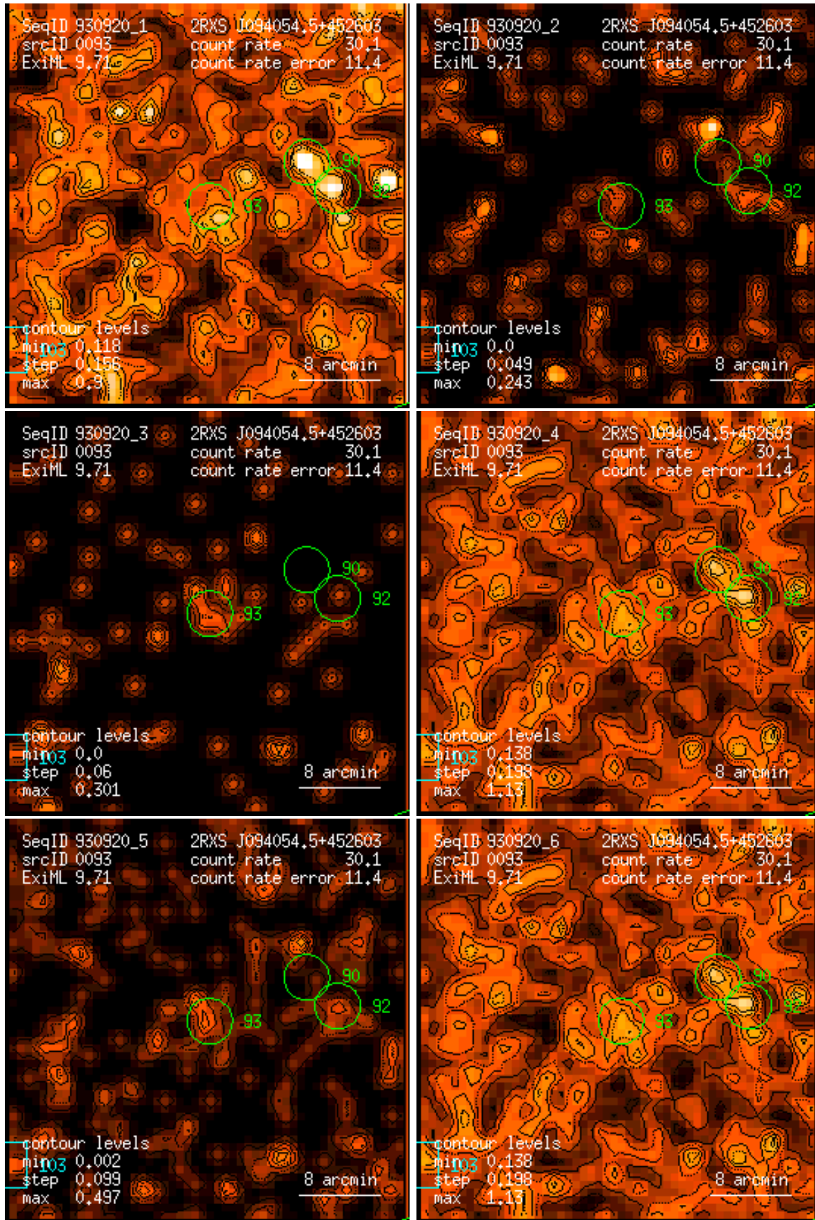
Figure 93: RASS 930920: detection 0093: band rate images, Gaussian filter: (1) PSPC channels 11 – 41, (2) 52 – 90, (3) 91 – 201, (4) 11 – 235, (5) 52 – 201, (6) 11 – 201. Broad band rates in counts/ks. Band rate contour levels in counts/ks/arcmin 2 .
