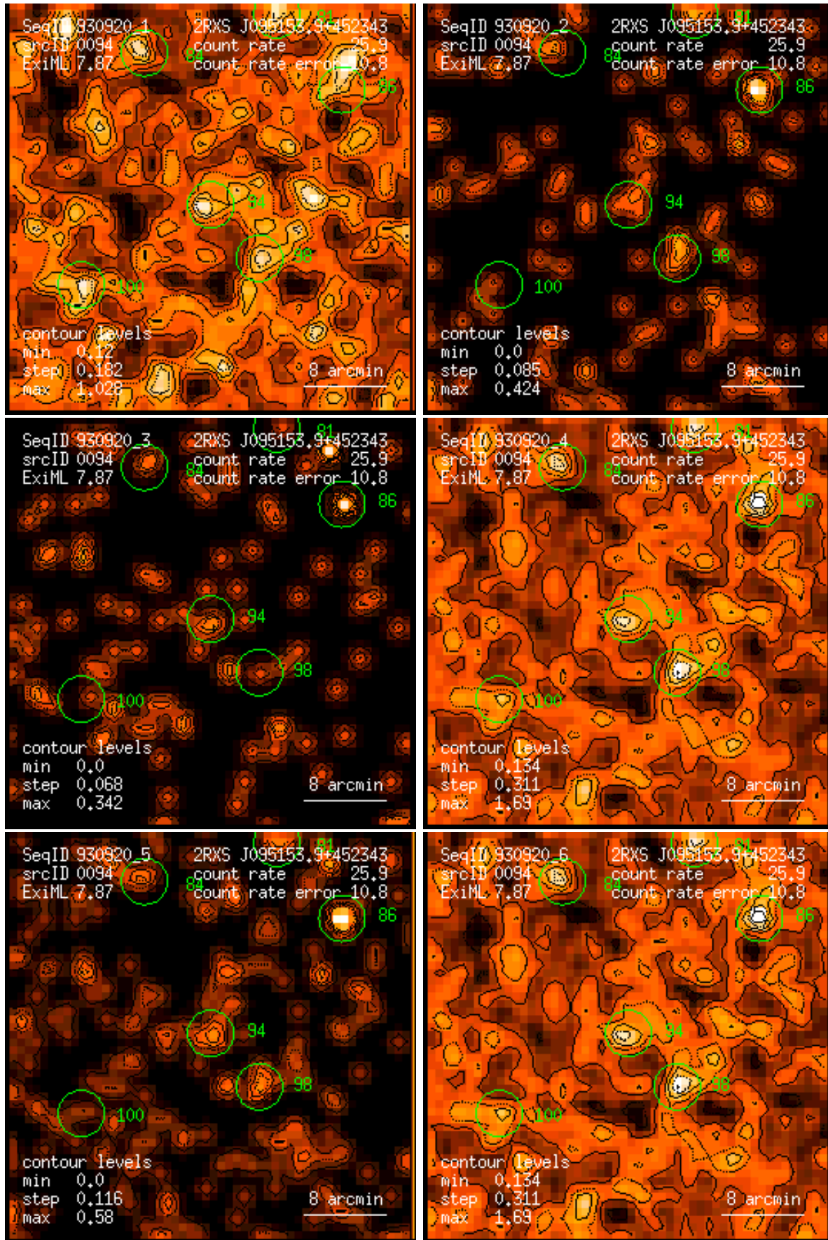
Figure 94: RASS 930920: detection 0094: band rate images, Gaussian filter: (1) PSPC channels 11 – 41, (2) 52 – 90, (3) 91 – 201, (4) 11 – 235, (5) 52 – 201, (6) 11 – 201. Broad band rates in counts/ks. Band rate contour levels in counts/ks/arcmin 2 .
